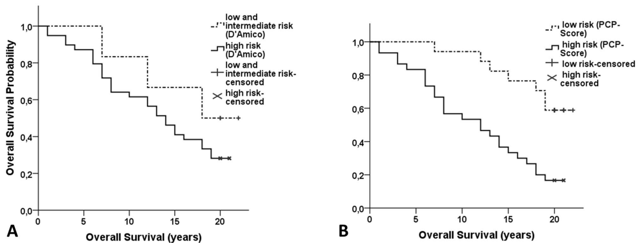
Figure 2. Overall Survival stratified according to (A) D'Amico classification: low and intermediate risk (GS \leq 7 and PSA \leq 20 ng/ml and \leq T2b ) versus high risk (GS > 7 or PSA > 20 ng/ml or \geq T3 ), p = 0.285 and (B) new PCP-Score: low risk (GS \leq 6 and genomic stability and high SATB1 expression in at least one tissue core) versus high risk (GS \geq 7 or genomic instability or low/negative SATB1 expression in all four obtained cores), p = 0.001 ; P -values for the log-rank test.
