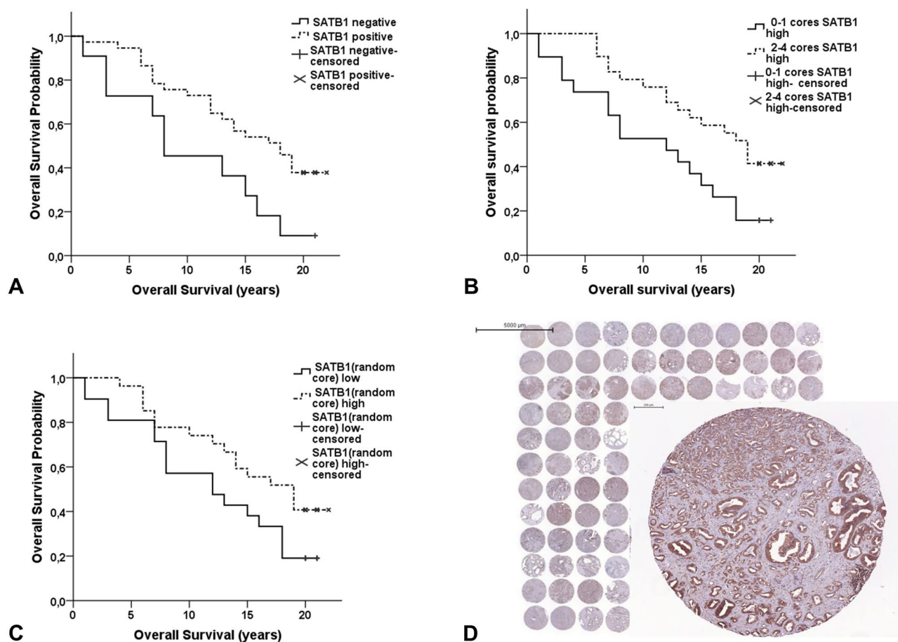
Figure 1. Overall Survival stratified by (A) at least one tissue core with a high SATB1 expression per tumor (SATB1 positive), p = 0.02 ; (B) the number of tissue cores with a high SATB1 expression per tumor, p = 0.018 ; (C) and the SATB1 expression in one randomly chosen tissue core per tumor, p = 0.068 ; (D) TMA slide with SATB1 stained tissue cores (one TMA tissue core enlarged). P-values for the log-rank test.
