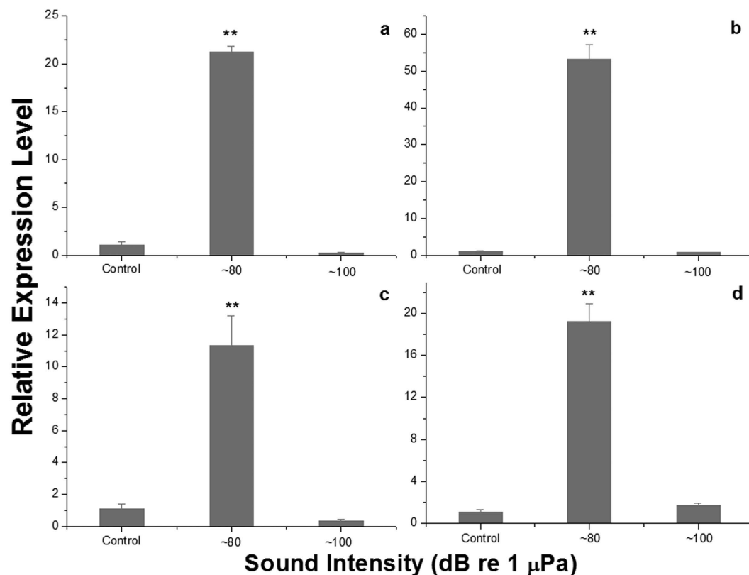
Figure 3. Relative gene expression levels for different sound intensity groups. Relative gene expression levels (mean \pm SE) of 6-phosphofructokinase-1 (a), pyruvate kinase (b), acetyl-CoA carboxylase (c), and arylformamidase (d) in razor clams exposed to one week of ambient sound or to ~80 dB re 1 \mu Pa or ~100 dB re 1 \mu Pa of underwater sounds (* and ** indicate a significant and an extremely significant difference by t-test, respectively, relative to the control of ambient sound).
