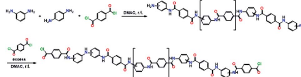
Scheme 1 Synthesis of the aramid oligomers.
