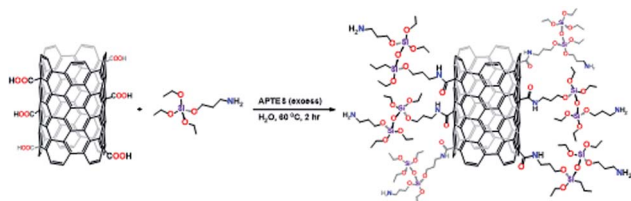
Scheme 2 Synthesis of the silanized carbon nanotubes (CNTs).
