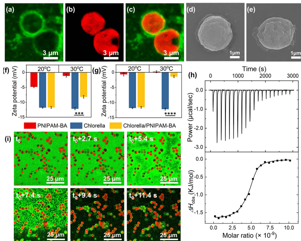
Fig. 2 Interaction mechanism between Chlorella and PNIPAM-co-BA. CLSM images of Chlorella /PNIPAM-co-BA complexes with 0.5 wt% PNIPAM-co-BA and 7.55 \times 10^7 cells per mL Chlorella at 30 °C. (a) The green fluorescence is from the fluorescently labeled PNIPAM-co-BA. (b) The red fluorescence is from intracellular chlorophyll. (c) is an overlay of (a) and (b). Scale bars, 3 \mu\text{m} . SEM images of Chlorella alone (d) and Chlorella /PNIPAM-co-BA (e) at 30 °C. Scale bars, 1 \mu\text{m} . Zeta potentials of PNIPAM-co-BA, Chlorella , Chlorella /PNIPAM-co-BA at 20 °C and at 30 °C with different PNIPAM-co-BA concentrations: ((f) 0.0125 wt%, (g) 0.1 wt%) ( n = 3 , mean \pm SD). (h) ITC results of raw and integrated data of released heat for titration of Chlorella suspension to PNIPAM-co-BA solution at 30 °C. (i) Time-lapse confocal fluorescence images demonstrate the enrichment of PNIPAM-co-BA on the surface of Chlorella during in situ heating. In this study, a low concentration of 0.5 wt% PNIPAM-co-BA was specially used to avoid the formation of gel affecting the visualization of the images. Scale bars, 25 \mu\text{m} .
