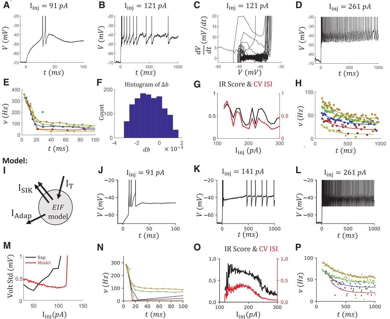
Figure 8. Reproducing the OB, IR firing patterns, and adaption simultaneously in a VIP cell model. A–D , Voltage traces at I_{inj} = 91, 121, 261 pA, which are examples to show OB, IR, and Adap, respectively. E , The instantaneous firing rates \nu from 0 to 100 ms that show the OB. Colors represent sweeps with different injection currents I_{inj} = 91, 131, 171, 212, 251, 291 pA. F , The histogram of \Delta b with an initial value b_{init} = 0.25 . The average change is \langle \Delta b \rangle = -0.0009 . G , The ISI ratio (black) and CV ISI (red) curves that show the irregularity. H , The instantaneous firing rates \nu between 100 ms and 1 s that show the Adap. Color coding is the same as in D . I , Sketch of the VIP cell model. J–P , Corresponding modeling results. M , SD of the voltage of the data and the model.
