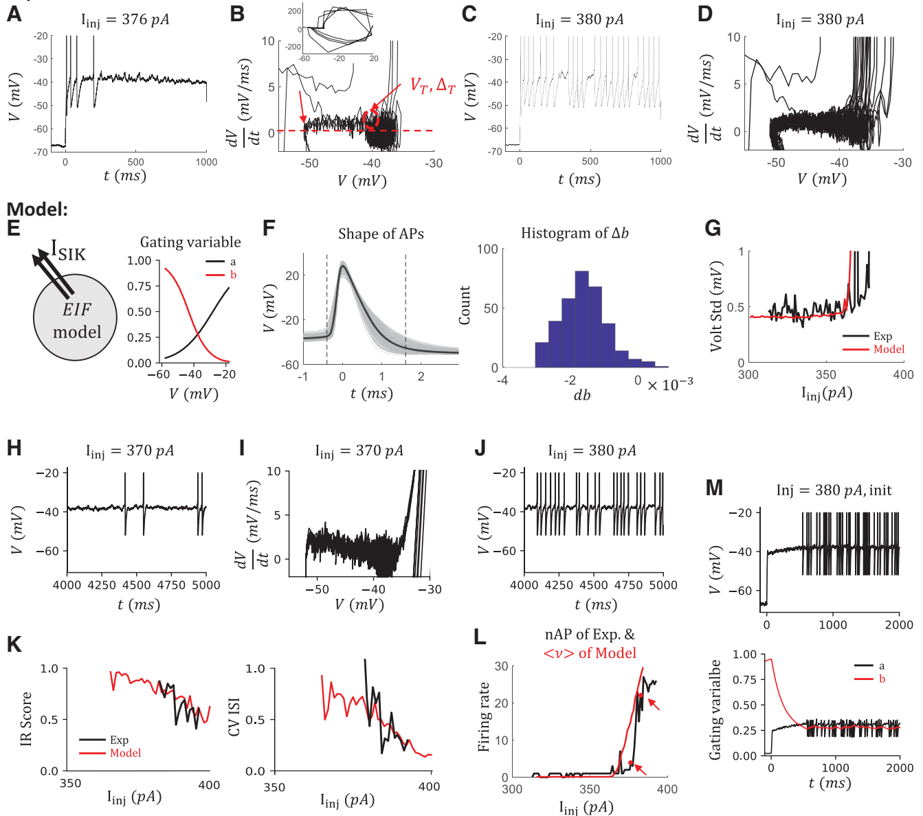
Figure 3. Modeling IR spiking of a canopy cell with an SIK channel. A , The voltage trace of an example canopy cell at I_{inj} = 376 pA. B , Phase diagram of the cell. Inset, The corresponding zoom-out diagram. y axis is the slope of the voltage trace, which is proportional to the net current to the cell. Red arrows indicate where we estimate the value of reset, curvature, and firing threshold of the corresponding model. C , D , The trace and the phase diagram at I_{inj} = 380 pA. E , The sketch of the canopy cell model (left) and the equilibrium value of the gating variables of the SIK channel (right). F , \Delta b estimation. Left, The shapes of all the APs from all the sweeps of the same cell. We exclude the first two APs in every sweep. APs are aligned at the maximum of the voltage. Dashed lines indicate t = -0.4, 1.6 ms, respectively. Voltage traces of these 2 ms time windows are used to calculate the jump of the slow inactivation variable \Delta b . Right, The histogram of \Delta b with an initial value b_{init} = 0.28 . The value b_{init} = 0.28 is the average value after 3 s of injection in the simulation. The average change is \langle \Delta b \rangle = -0.0020 . G , The voltage SD measured between 500 ms and 1 s during the current injection from the data (black) and the model (red). H , I , The voltage trace and the phase diagram of the canopy cell model at I_{inj} = 370 pA. J , The voltage trace at I_{inj} = 380 pA. K , The comparison of irregularity from the data and the model by IR score (left) and by CV ISI (right). L , The comparison of firing rate from the data, estimated by the number of APs during the 1 s current injection, and from the model, estimated by the steady-state firing rate. Red arrows indicate I_{inj} = 376, 380 pA. M , The initial dynamics are not considered in this model. Top, The voltage trace that includes the initial transient part when I_{inj} = 380 pA. Bottom, The transient dynamics of gating variables of the SIK channel. Black and red lines indicate the fast and slow variables a and b , respectively.
