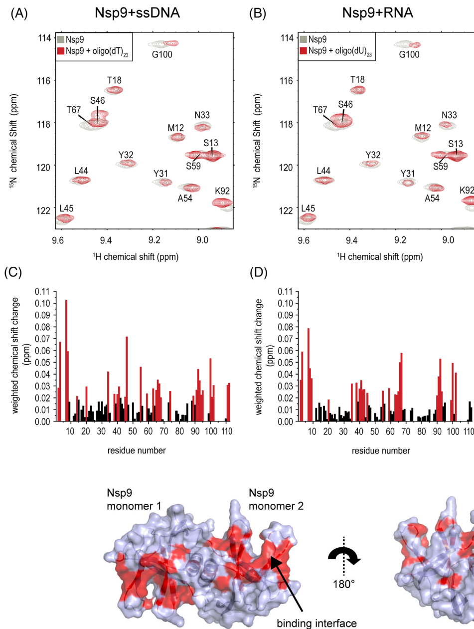
FIGURE 5 NMR reveals distinct interaction surface. Nsp9 dimer structure (taken from PDB 6WXD) in surface and cartoon representation (colored in light blue). The RNA binding residues as determined in Figure 4C,D were mapped onto the deposited crystal structure. (red). Note that a distinct binding interface exists on one side of the dimer structure
