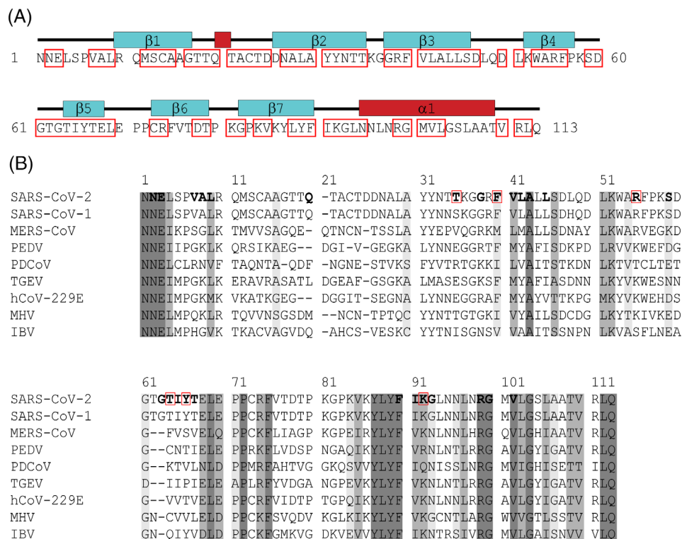
FIGURE 1 Coronavirus family Nsp9 sequence information.
