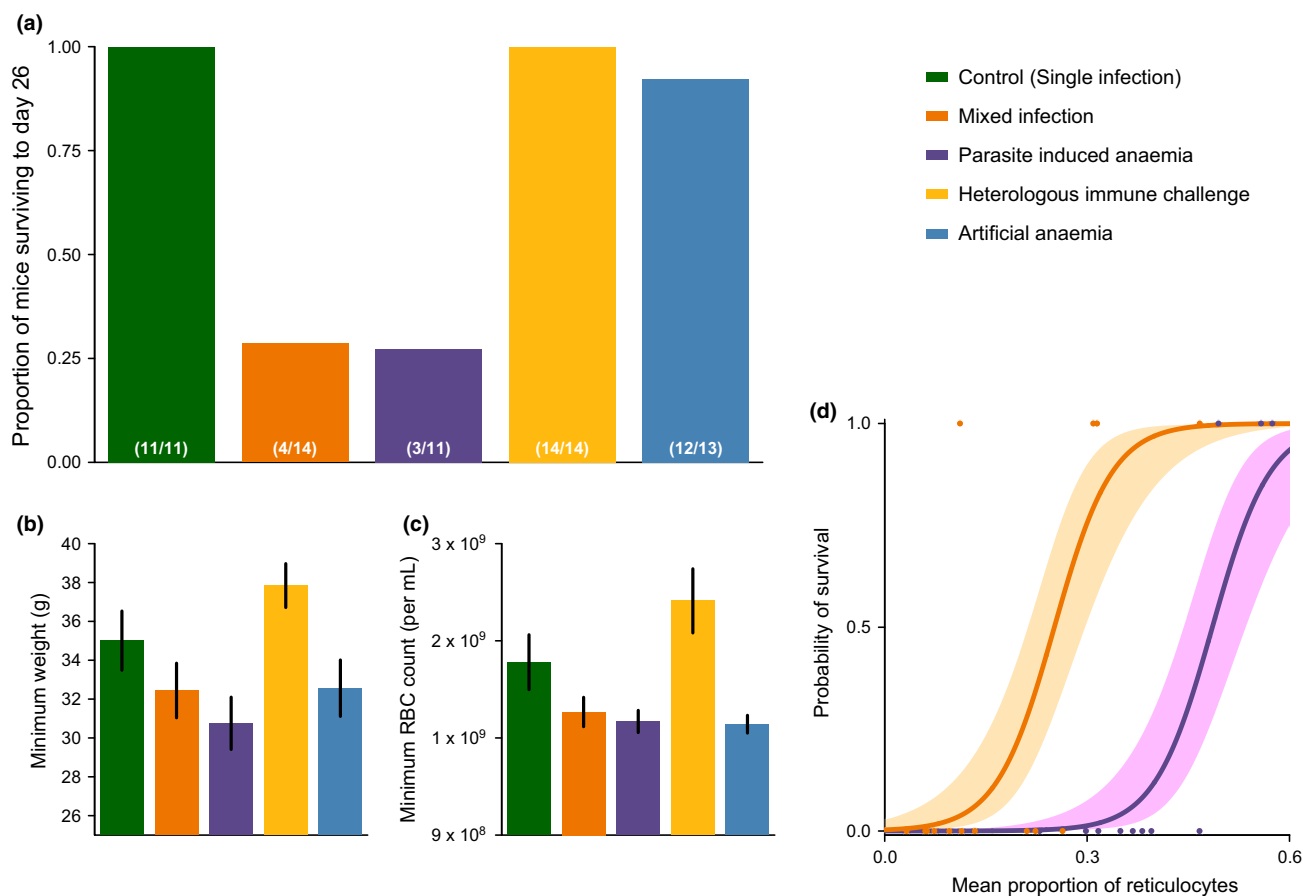
Figure 4 Co-infections of a RBC generalist and RBC specialist are more virulent to the host. Panels (a, b and c) show the proportion surviving mice, minimum weight and minimum red blood cell count for the five treatment groups, respectively. Panel d shows the relationship between mean proportion of reticulocytes and survival for the two treatments where substantial mortality was experienced (mixed infections, orange, and parasite-induced anaemia, purple).
