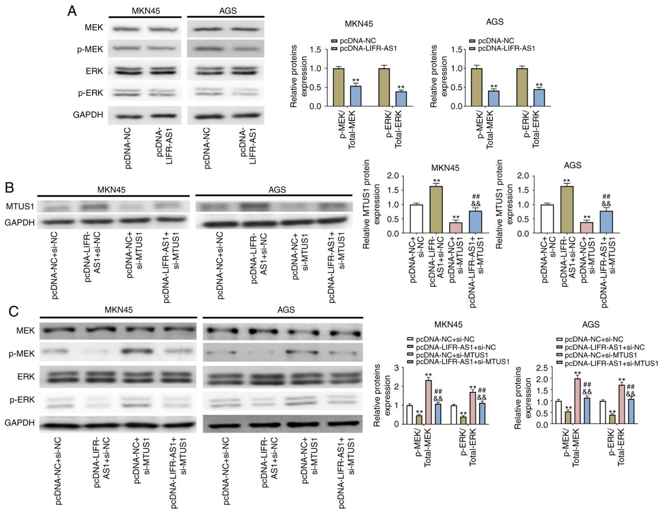
Figure 5. Overexpression of lncRNA LIFR-AS1 blocks the MEK/ERK pathway by regulating MTUS1. (A) The vectors of pcDNA-LIFR-AS1 and pcDNA-NC were transfected into GC (MKN45 and AGS) cell lines and the protein levels of p-MEK/MEK and p-ERK/ERK were examined using western blotting. (B) The expressed vectors of pcDNA-LIFR-AS1 and si-MTUS1 as well as the corresponding controls (pcDNA-NC and si-NC) were transfected into GC (MKN45 and AGS) cell lines and the expression of MTUS1 in the transfected cells examined using western blotting. (C) The vectors of pcDNA-LIFR-AS1, si-MTUS1 and the corresponding controls (pcDNA-NC and si-NC) were transfected into GC (MKN45 and AGS) cell lines and protein levels of p-MEK/MEK and p-ERK/ERK were examined using western blotting. ** P < 0.01 vs. pcDNA-NC group, ## P < 0.01 vs. pcDNA-LIFR-AS1+si-NC group, && P < 0.01 vs. pcDNA-NC+si-MTUS1 group. Inc., long non-coding; MTUS1, microtubule-associated tumor suppressor 1; si, small interfering; NC, negative control; GC, gastric carcinoma; p-, phosphorylated.
