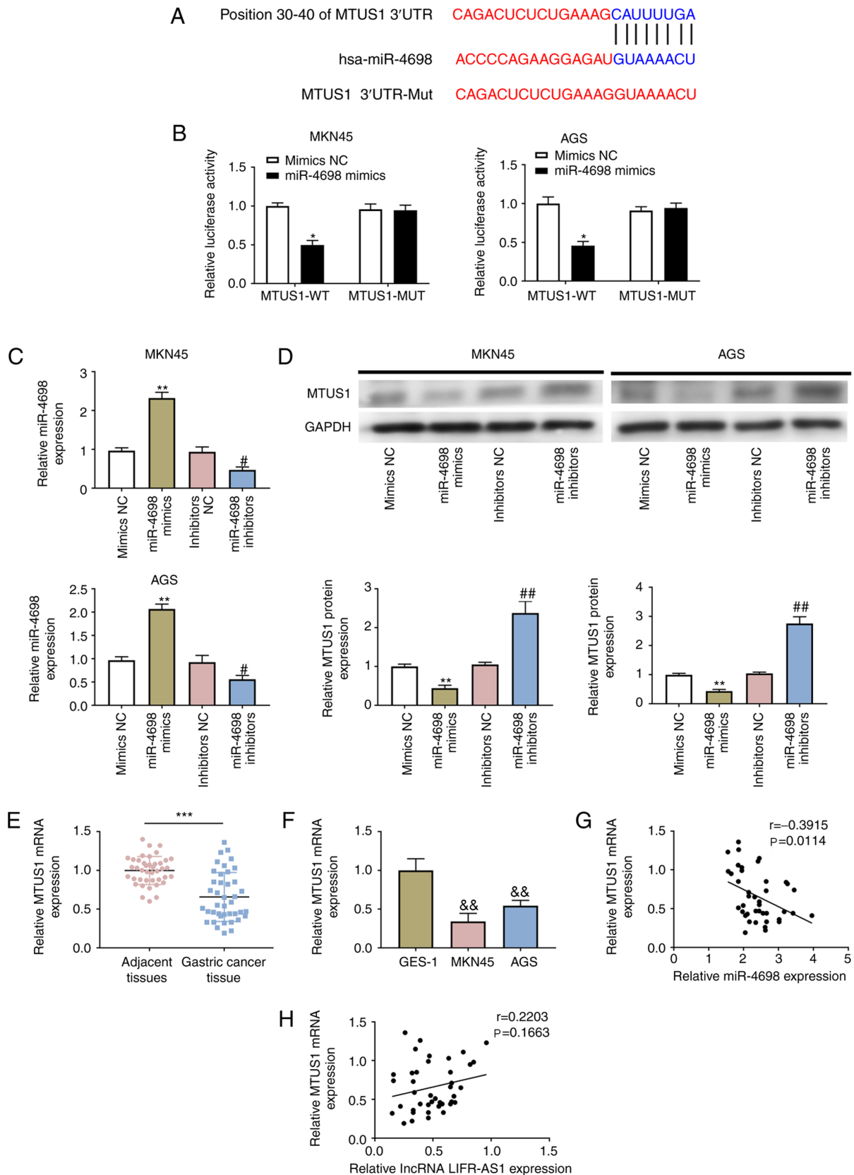
Figure 4. MTUS1 is a direct target of miR-4698 and is positively regulated by lncRNA LIFR-AS1. (A) The binding sequence between miR-4698 and MTUS1 was predicted using TargetScan algorithms. (B) Association between MTUS1 and miR-4698 was evaluated using a luciferase reporter system. The vectors of miR-4698 mimics and miR-4698 inhibitors as well as the corresponding controls (mimics NC and inhibitors NC) were transfected into GC (MKN45 and AGS) cell lines. (C) The expression of miR-4698 in above transfected cells was explored using RT-qPCR; (D) The expression of MTUS1 in above transfected cells was evaluated using western blotting. Expression of MTUS1 in (E) 41 pairs of GC tissues and matched adjacent tissues and (F) in GES-1 and GC (MKN45 and AGS) cell lines was examined using RT-qPCR. Interactions between MTUS1 and (G) miR-4698 or (H) lncRNA LIFR-AS1 were investigated using Pearson correlation analysis. * P < 0.05 vs. MTUS1-WT+Mimics NC group, ** P < 0.01 vs. Mimics NC group, && P < 0.01 vs. GES-1 group, *** P < 0.001 vs. adjacent tissues group, # P < 0.05 vs. inhibitors NC group, ## P < 0.01 vs. inhibitors NC group. MTUS1, microtubule-associated tumor suppressor 1; miR, microRNA; Inc, long non-coding; NC, negative control; GC, gastric carcinoma; GES-1, gastric mucosal epithelial cell line; RT-qPCR, reverse transcription-quantitative PCR.
