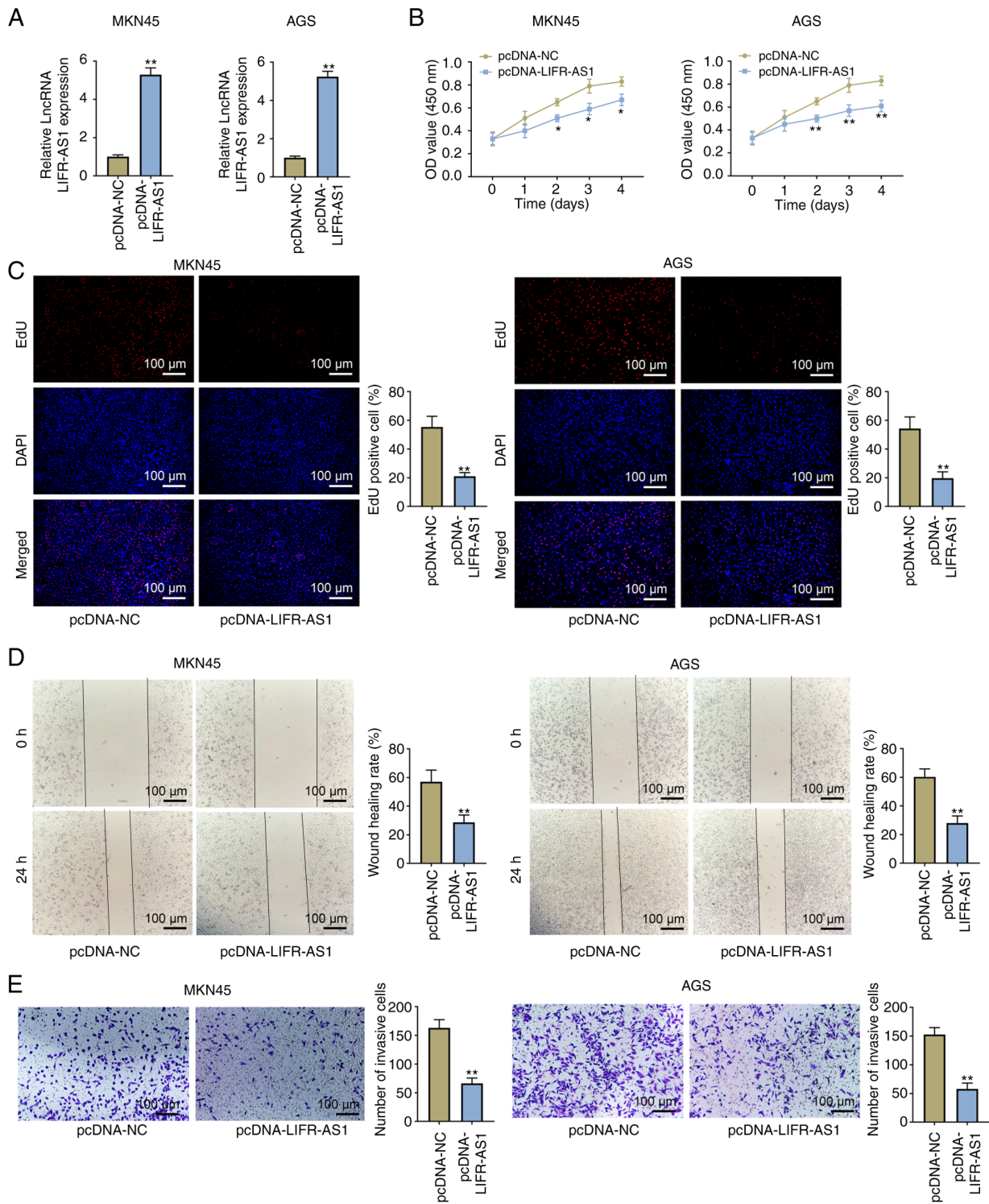
Figure 2. Overexpressed lncRNA LIFR-AS1 inhibits GC cell proliferation and migration. (A) Expression of lncRNA LIFR-AS1 in pcDNA-LIFR-AS1 and pcDNA-NC transfected GC (MKN45 and AGS) cell lines was explored using reverse transcription-quantitative PCR. After successful transfection, the proliferative abilities of MKN45 and AGS cells were assessed by (B) CCK-8 and (C) EdU; the migration capacities of MKN45 and AGS cells were evaluated using (D) wound healing and (E) Transwell invasion assays. Scale bar=100 \mu m. * P <0.05, ** P <0.01 vs. pcDNA-NC group. lnc, long non-coding; GC, gastric carcinoma; NC, negative control; EdU, 5-ethynyl-2'-deoxyuridine.
