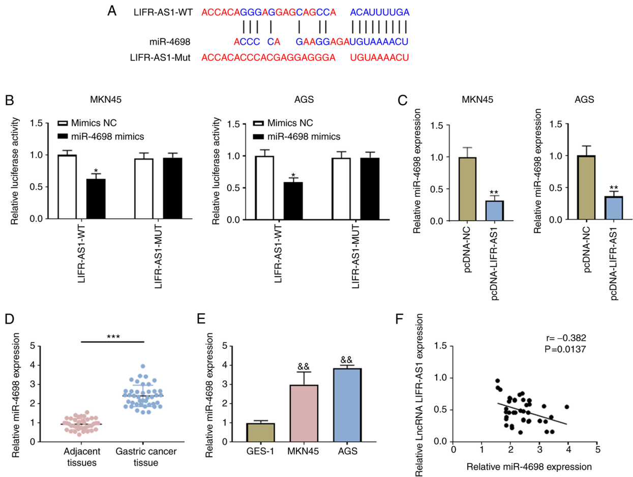
Figure 3. lncRNA LIFR-AS1 acts as a sponge for miR-4698. (A) The sequence of binding site between lncRNA LIFR-AS1 and miR-4698 was predicted using the online tool DIANA. (B) Association between lncRNA LIFR-AS1 and miR-4698 was investigated using a luciferase reporter system. (C) Expression of miR-4698 was established following pcDNA-LIFR-AS1 and pcDNA-NC transfection using RT-qPCR. Expression of miR-4698 in (D) 41 pairs of GC tissues and matched adjacent tissues and (E) in GES-1 and GC (MKN45 and AGS) cell lines was evaluated using RT-qPCR. (F) Mutual regulation between lncRNA LIFR-AS1 and miR-4698 was assessed using Pearson correlation analysis. * P < 0.05 LIFR-AS1-WT+Mimics NC group, ** P < 0.01 vs. pcDNA-NC group, && P < 0.01 vs. GES-1 group, *** P < 0.001 vs. adjacent tissues group. Inc., long non-coding; miR, microRNA; RT-qPCR, reverse transcription-quantitative PCR; GC, gastric carcinoma; GES-1, gastric mucosal epithelial cell line; Wt, wild type; Mut, mutant; NC, negative control.
