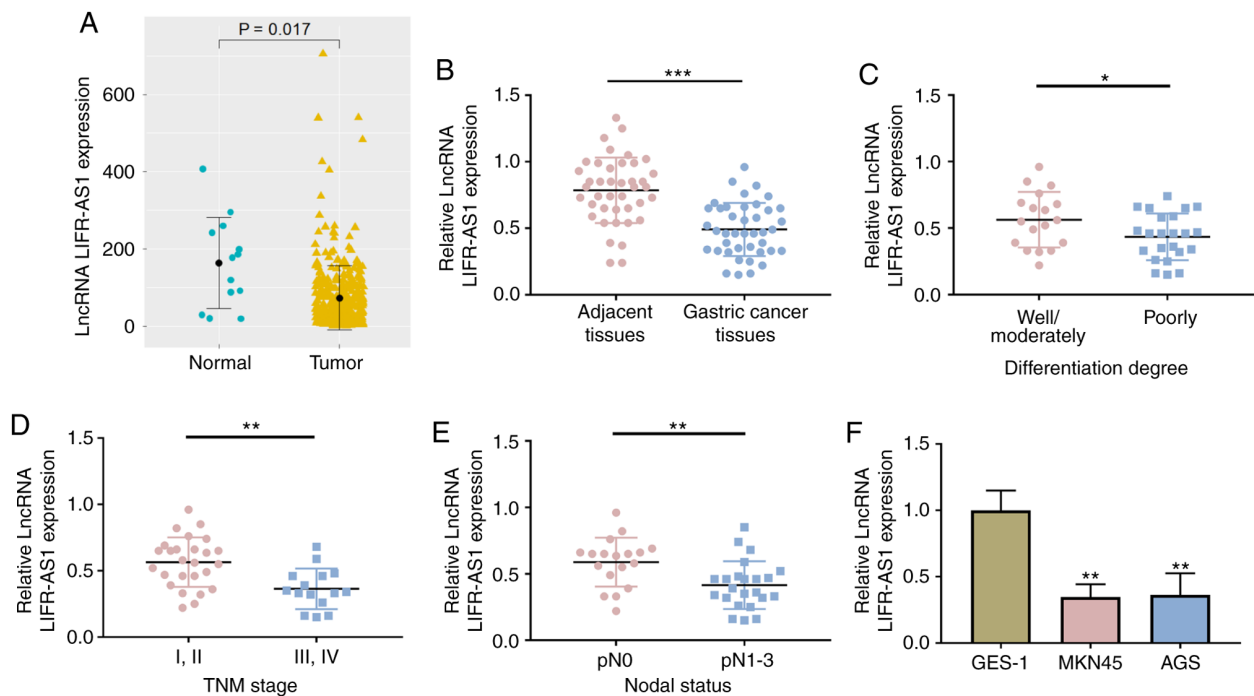
Figure 1. Decreased lncRNA LIFR-AS1 expression in GC tissues and cell lines. (A) Expression of lncRNA LIFR-AS1 in GC tissues and normal tissues were downloaded from the TCGA database. (B) Expression of lncRNA LIFR-AS1 in 41 pairs of GC tissues and matched adjacent tissues was determined using RT-qPCR. Expression of lncRNA LIFR-AS1 in 41 patients with GC with the condition of (C) well/moderately and poorly differentiation, (D) different TNM stages and (E) pN0-3 nodal status was investigated using RT-qPCR. (F) Expression of lncRNA LIFR-AS1 in GES-1 and GC (MKN45 and AGS) cell lines was assayed using RT-qPCR. * P < 0.05 , ** P < 0.01 , *** P < 0.001 . Inc, long non-coding; GC, gastric carcinoma; TCGA, The Cancer Genome Atlas; RT-qPCR, reverse transcription-quantitative PCR; GES-1, gastric mucosal epithelial cell line.
