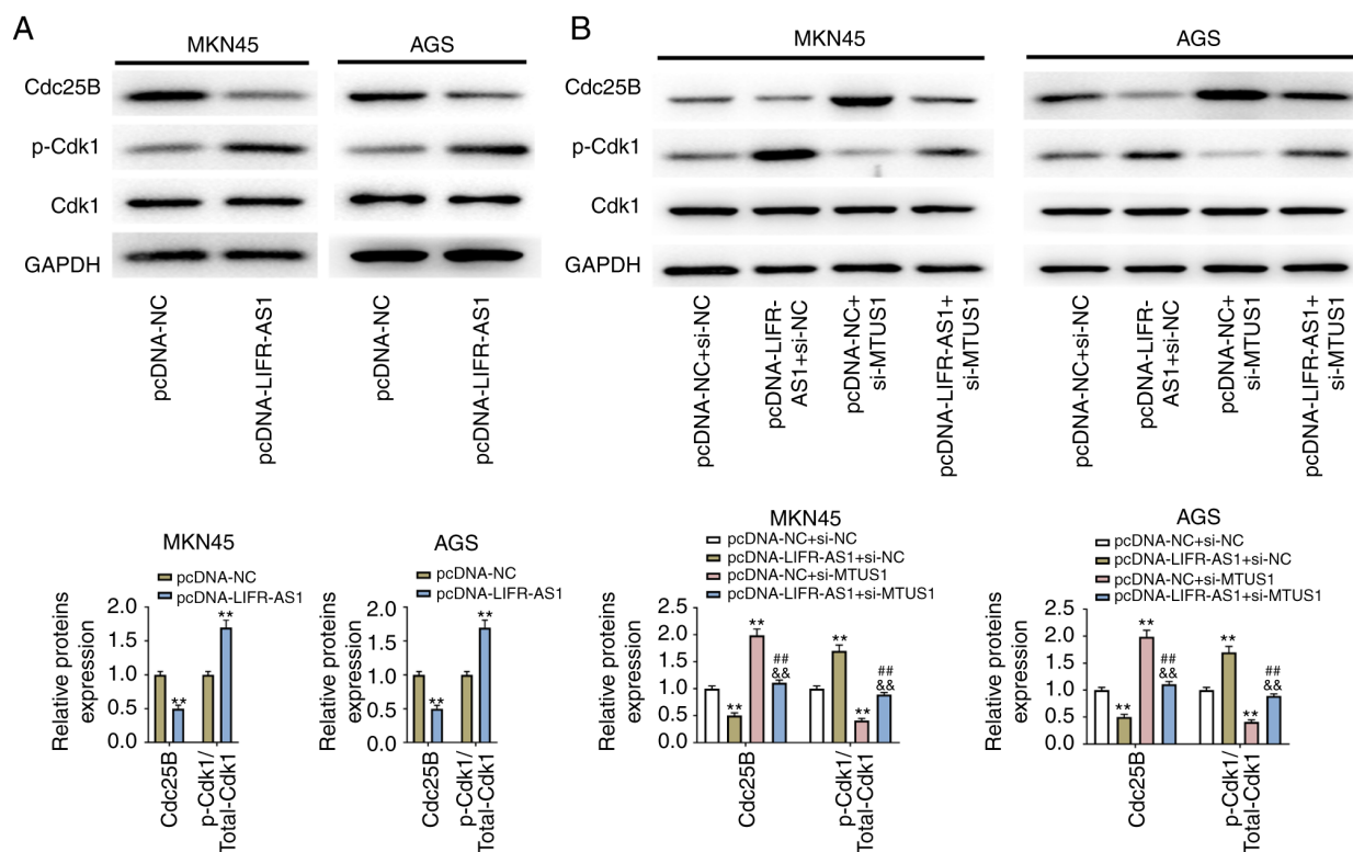
Figure 6. Overexpression of lncRNA LIFR-AS1 inhibits Cdc25B and inactivates Cdk1 signaling. (A) The vectors of pcDNA-LIFR-AS1 and pcDNA-NC were transfected into GC (MKN45 and AGS) cell lines, protein levels of Cdc25B and p-Cdk1 were examined using western blotting. (B) The vectors of pcDNA-LIFR-AS1, si-MTUS1 and the corresponding controls (pcDNA-NC and si-NC) were transfected into GC (MKN45 and AGS) cell lines, protein levels of Cdc25B and p-Cdk1 were examined using western blotting. ** P < 0.01 vs. pcDNA-NC group, ## P < 0.01 vs. pcDNA-LIFR-AS1+si-NC group, && P < 0.01 vs. pcDNA-NC+si-MTUS1 group. lnc, long non-coding; Cdc, cell division cycle; Cdk, cyclin-dependent kinase; NC, negative control; GC, gastric carcinoma; si, small interfering; MTUS1, microtubule-associated tumor suppressor 1.
