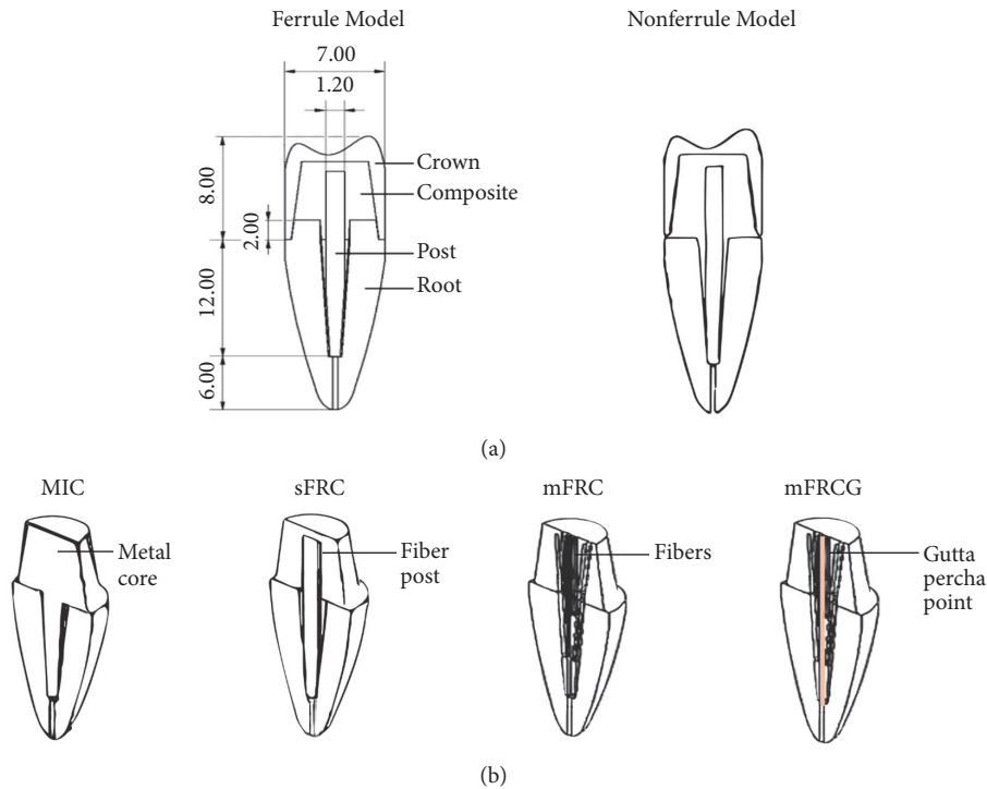
FIGURE 1: Representative figures of the models used in the study. Profile views of the ferrule and nonferrule models (a). Three-quarter view of the four different coronoradicular reconstructions (CRR): MIC (metal inlay core), single-fiber-reinforced composite (sFRC), multi-fiber-reinforced composite (mFRC), and multi-fiber-reinforced composite with gutta (mFRCG) for nonferrule models (b). Dimensions are in mm.
