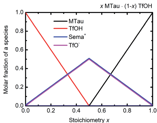
Fig. 4 Molar fractions of the species [2-Sema] + , MTau, TfOH and [TfO] − as a function of the stoichiometry x for the samples x MTau · (1 − x )TfOH. The curves of [2-Sema] + and [TfO] − coincide.
