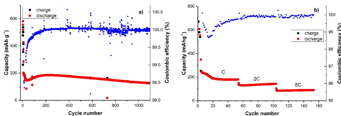
Figure 7. Capacity vs. cycle number at: (a) 1C rate for 1100 cycles; and (b) at 1C, 2C and 5C current rate for 50 cycles each.
