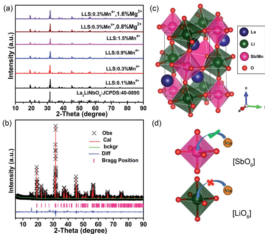
Fig. 1 (a) XRD patterns of the LLS: x\text{Mn}^{4+}, y\text{Mg}^{2+} phosphors. (b) Rietveld refinement XRD pattern of the LLS: 0.3\%\text{Mn}^{4+} phosphors. (c) The structure of the LLS: 0.3\%\text{Mn}^{4+} phosphors. (d) The octahedron configuration diagrams of [\text{SbO}_6] and [\text{LiO}_6] .
