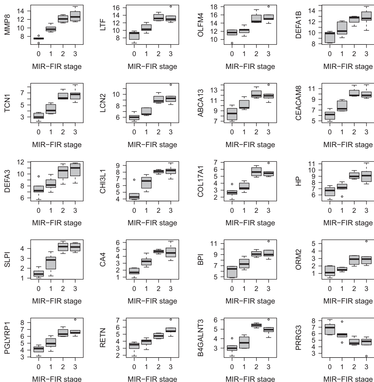
Fig. 9. Combined MIR and FIR linear effect on gene expression. Top-20 genes with largest fold change among DE genes with FDR < 5% and minimum 50%-fold change throughout the following combined 4 stages of MIR and FIR: 0 no MIR and no FIR; 1 MIR but no FIR; 2 MIR stage 3 and FIR stage 1; 3 MIR stage 3 and FIR stage 2 or 3. Adjusted expression values in log-CPM units are plotted in the y-axis as function of the combined stages in the x-axis. In the boxplots, the horizontal solid line indicates the median, the box limits correspond to the 25th and 75th percentile that span the IQR, while the whiskers, or error bars, extend to 1.5 times the IQR away from the median and values exceeding that distance, if any, are depicted by open circles.
