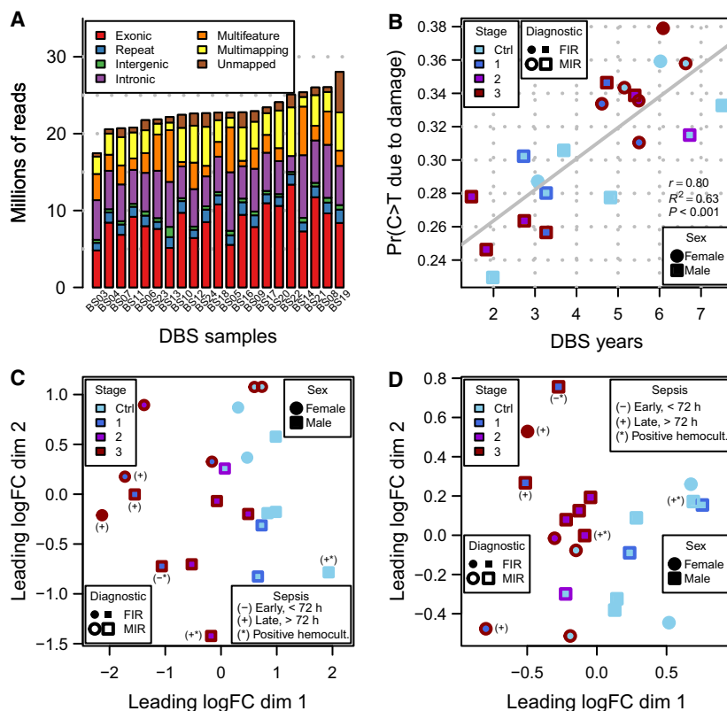
Fig. 2. Transcriptomics and proteomics profiling of archived DBSs. (A) Sequencing depth per sample, broken by origin of sequence reads. (B) Probability of a C > T deamination due to damage, as function of DBS age in years. (C) Sample differences in terms of fold changes between transcriptomic samples in base-2 logarithmic scale (logFC), projected along the x- and y-axes. Distance between points is proportional to the dissimilarity between samples. (D) Same as (C) but calculated from proteomic samples.
