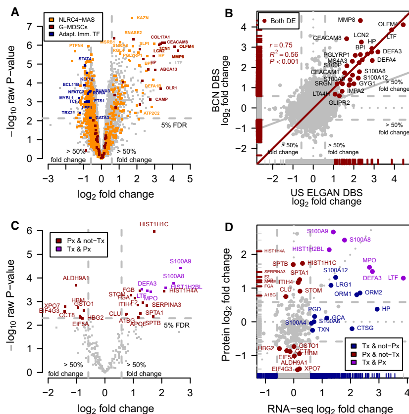
Fig. 3. Differential expression analysis between FIR-affected and unaffected ELGANs, of transcriptomic and proteomic profiles from archived DBSs. (A) Volcano plot of transcriptomics data. Raw P values in negative logarithmic scale on the y-axis as a function of the \log_2 -fold change on the x-axis. Orange dots highlight genes from a NLR4-MAS signature [16], red dots highlight genes from a G-MDSCs signature [17], and blue dots highlight transcription factor coding genes involved in regulating adaptive immunity. (B) Fold changes of this study on the y-axis as a function of fold changes in data from the US ELGAN cohort in the x-axis. (C) Volcano plot of proteomics data. (D) Fold changes from proteomics data on the y-axis as a function of fold changes from transcriptomics data on the x-axis.
