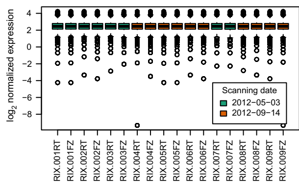
Fig. 5. Distribution of background-corrected and quantile-normalized expression values from the US ELGAN cohort microarray data. In the boxplots, the horizontal solid line indicates the median, the box limits correspond to the 25th and 75th percentile that span the IQR, while the whiskers, or error bars, extend to 1.5 times the IQR away from the median and values exceeding that distance, if any, are depicted by open circles.
