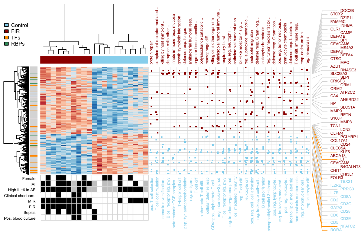
Fig. 8. FIR gene expression signature and functional enrichment analysis. Heatmap of expression values for 782 DE genes with FDR < 5% and minimum 1.5-fold change between FIR-affected and unaffected ELGANS, obtained after removing FIR-unrelated variability. Dendrograms on the x- and y-axes represent the hierarchical clustering of samples and genes, respectively. Leaves on the gene dendrogram are color coded according to whether genes encode for transcription factors (orange) or RNA-binding proteins (green), while those on the sample dendrogram are color coded according to FIR status, where red indicates samples derived from FIR-affected infants and blue unaffected. The right dot-matrix represents DE genes (y-axis) belonging to GO terms (x-axis) significantly enriched (FDR < 10% and odds ratio -OR > 1.5) by upregulated (top) and downregulated (bottom) DE genes. The bottom-left dot-matrix represents the presence or absence of phenotypes, with gray indicating missing data.
