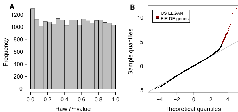
Fig. 7. Differential expression between FIR and non-FIR samples from the US ELGAN cohort microarray data. (A) Distribution of raw P -values (B) Quantile–quantile plot of moderated t -statistics. Red dots indicate differentially expressed genes with FDR < 5% and minimum 1.5-fold change.
