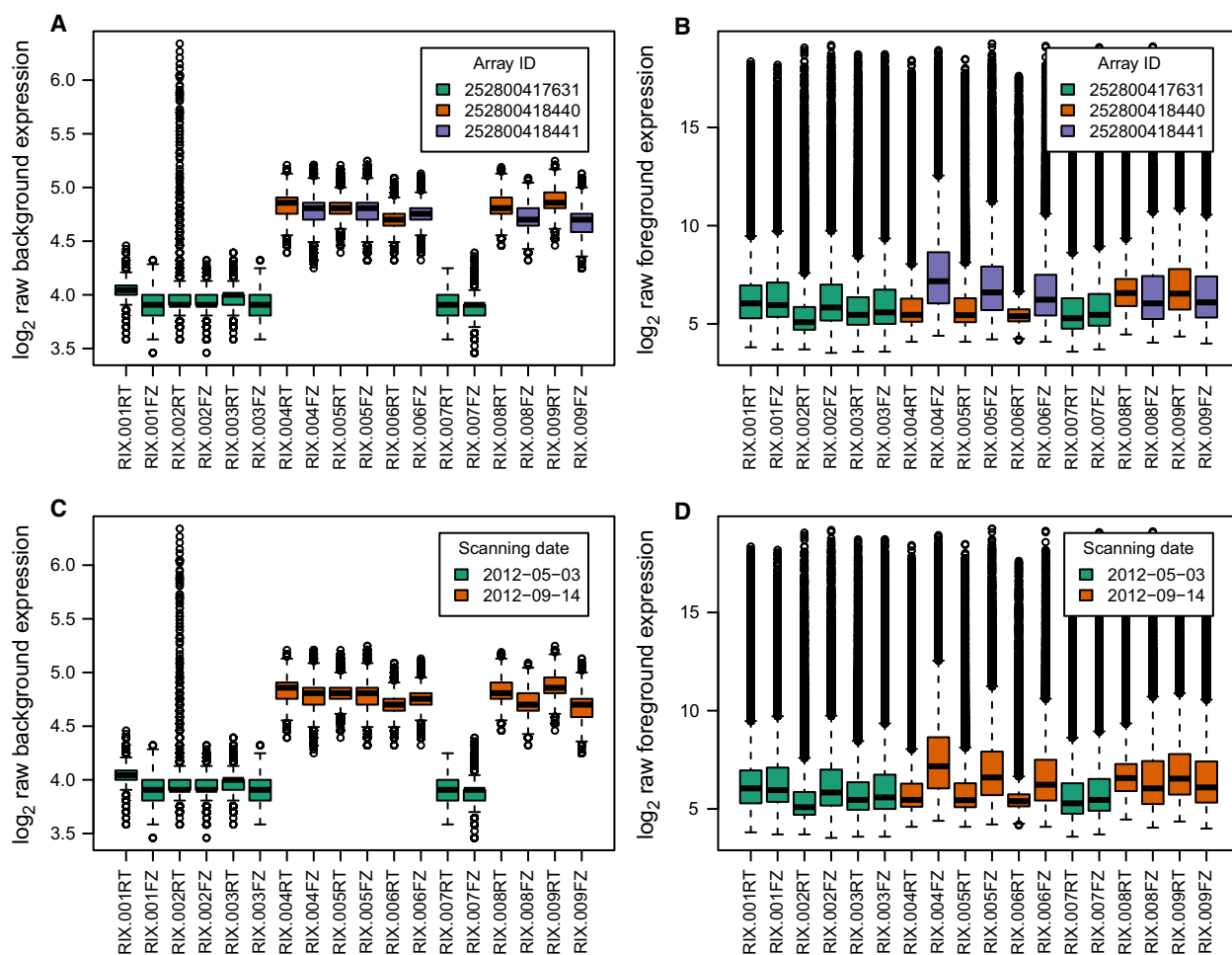
Fig. 4. Distribution of raw expression values from the US ELGAN cohort microarray data. (A, C) Expression values from background probes. (B, D) Expression values from foreground probes. (A, B) Samples colored by array identifier. (C, D) Samples colored by scanning date. In the boxplots, the horizontal solid line indicates the median, the box limits correspond to the 25th and 75th percentile that span the IQR, while the whiskers, or error bars, extend to 1.5 times the IQR away from the median and values exceeding that distance, if any, are depicted by open circles.
