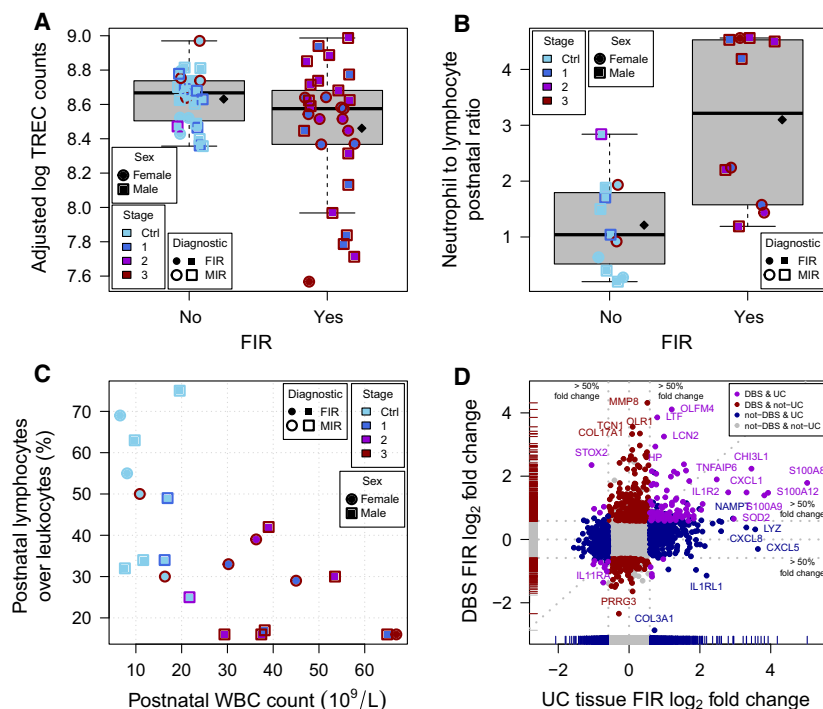
Fig. 10. Association of FIR with clinical and molecular signatures. (A) TREC-corrected fluorescent counts on logarithmic scale by FIR status, after adjusting for sex, maximum lymphocyte count during the first postnatal week and batch. Diamonds indicate mean values. There are multiple measurements per newborn. (B) Postnatal ratio of neutrophil absolute count to absolute lymphocyte count, during the first postnatal week, by FIR status. Diamonds indicate mean values. (C) Percent of all leukocytes that are lymphocytes during the first postnatal week on the y-axis as a function of the postnatal white blood cell count on the x-axis. (D) Fold changes in this study on the y-axis as a function of FIR fold changes in UC tissue on the x-axis. In the boxplots, the horizontal solid line indicates the median, the box limits correspond to the 25th and 75th percentile that span the IQR, while the whiskers, or error bars, extend to 1.5 times the IQR away from the median and values exceeding that distance, if any, are depicted by open circles.
