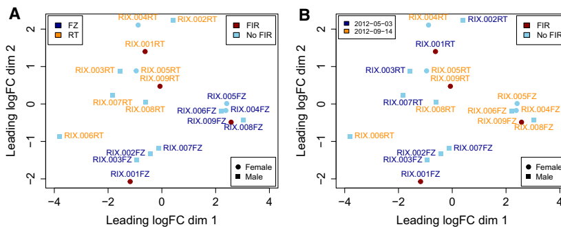
Fig. 6. Sample differences from the US ELGAN cohort microarray data, in terms of fold changes between samples in base-2 logarithmic scale. (A) Sample labels are colored by storage condition (FZ: frozen; RT: room temperature). (B) Sample labels are colored by microarray scanning date. There is a clear effect of storage condition, an effect of scanning date mostly in frozen samples and no apparent sex or FIR effect.
