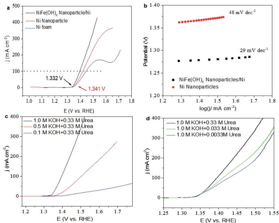
Fig. 4 (a) LSV curves of the NiFe(OH) x nanoparticles/Ni foam sample, the Ni/Ni foam and Ni foam in 1.0 M KOH electrolyte with 0.33 M urea at a scan rate of 10 mV s -1 . (b) Tafel plots of the NiFe(OH) x Nanoparticles/Ni foam sample and the Ni/Ni foam (c and d) LSV curves of different electrolyte and different urea concentration over the NiFe(OH) x nanoparticles/Ni foam sample.
