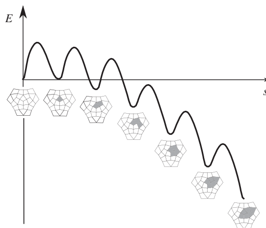
Figure 5. A typical energy cascade for the opening of the first 6 protomers in mode 2^- . The energy is plotted along a path in \mathbb{R}^{60} that is the union of the first 6 MEPs, and s is the arc parameter along the path.
