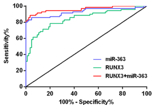
Figure 5. ROC curve of RUNX3 and miR-363 single test and combined diagnosis of colorectal cancer. The combined test of RUNX3 and miR-363 in peripheral blood has the highest sensitivity and specificity level, the area under the ROC curve (AUC) in the combined test is larger than the single test and has a higher diagnostic value. In the ROC curve, the combined test is closer to the upper left corner than the single test, and has a higher detection accuracy than the single test.
