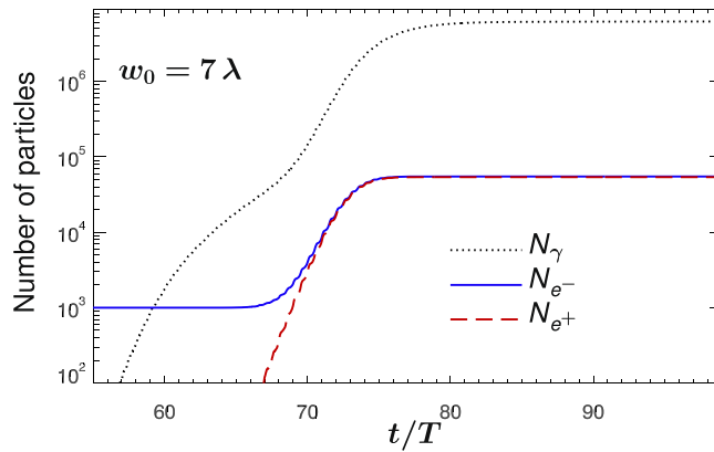
Figure 3. The evolution of the number of particles. The total number of electrons N_{e^-} (solid blue line), positrons N_{e^+} (dashed red line) and photons N_\gamma with energy \varepsilon_\gamma > 2.5 \text{ MeV} (dotted black line) as function of time t during the collision of two counter-propagating laser pulses. Time and space are in units of the laser period T = \lambda/c \approx 2.67 fs and laser wavelength \lambda = 0.8 \mu\text{m} , respectively. The two pulses have P = 500 PW power and w_0 = 7 \lambda waist radius, which imply an intensity I \approx 10^{24} \text{ W/cm}^2 . The initial 10^3 stray electrons originate from hydrogen.
