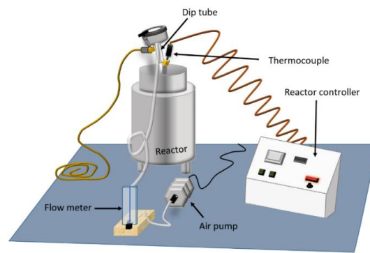
Figure 1. Equipment used to thermally oxidize engine oil.
