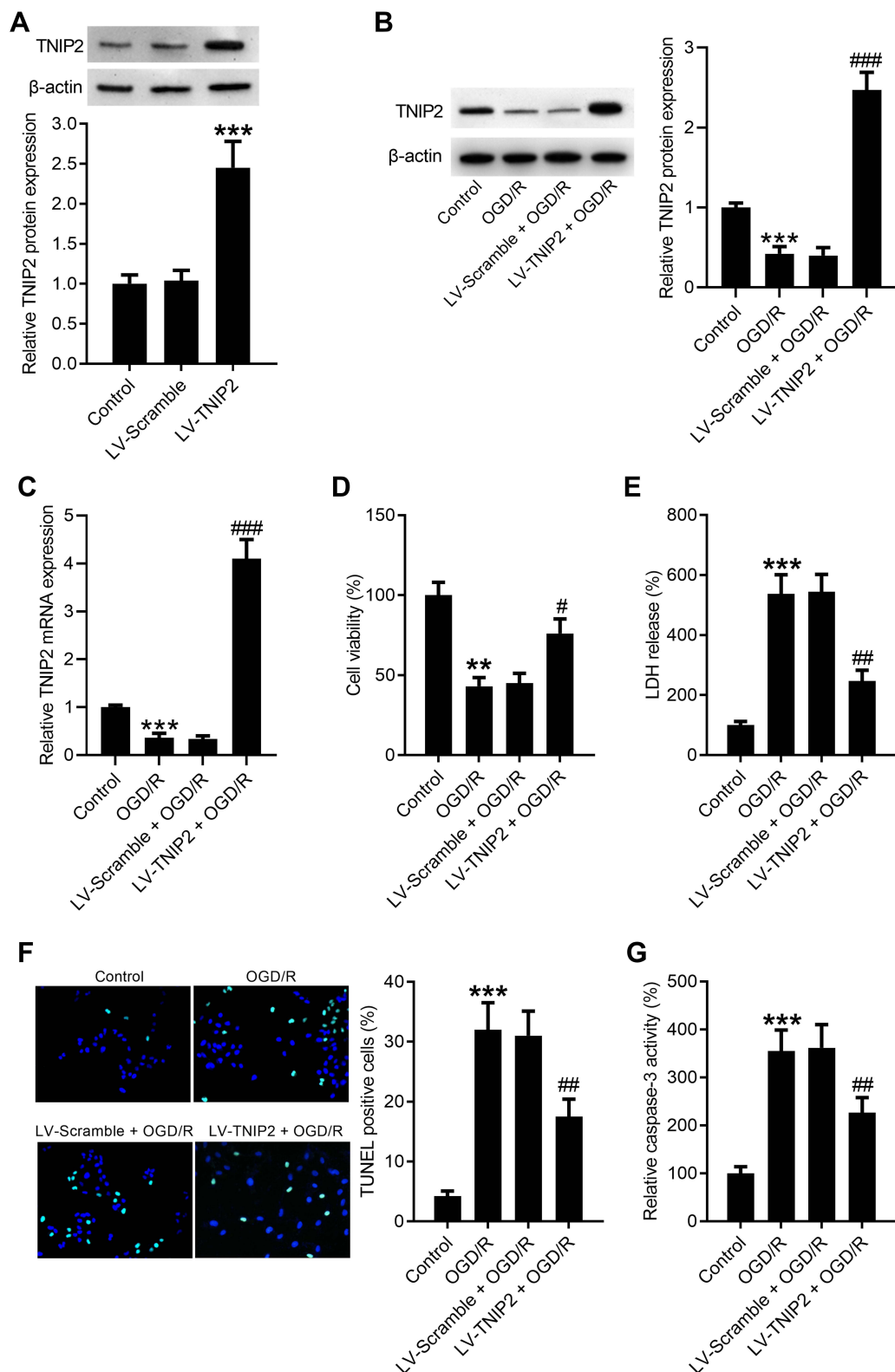
Figure 2 TNIP2 overexpression attenuates ODG/R-induced apoptosis in HT22 cells. (A) LV-Scramble and LV-TNIP2 were transfected into HT22 cells for 48 h and the transfection efficiency was confirmed using Western blot ( n = 3 ). HT22 cells were transfected with LV-TNIP2 or LV-Scramble, followed by exposure to ODG/R. (B and C) The expression levels of TNIP2 protein and mRNA were detected by Western blot and qRT-PCR, respectively. (D) The viability of HT22 cells was examined using CCK-8 assay ( n = 3 ). (E) The viability of HT22 cells was determined by measurement of LDH release ( n = 3 ). (F) Representative images of TUNEL staining were shown and the bar graph represents the quantification of TUNEL positive cells ( n = 3 ). (G) Caspase-3 activity assay kit was applied to examine the activity of caspase-3 ( n = 3 ). **P < 0.01 and ***P < 0.001 , compared with the LV-Scramble or control group. \#P < 0.05 , ##P < 0.01 , and ###P < 0.001 , compared with the LV-Scramble + ODG/R group.
