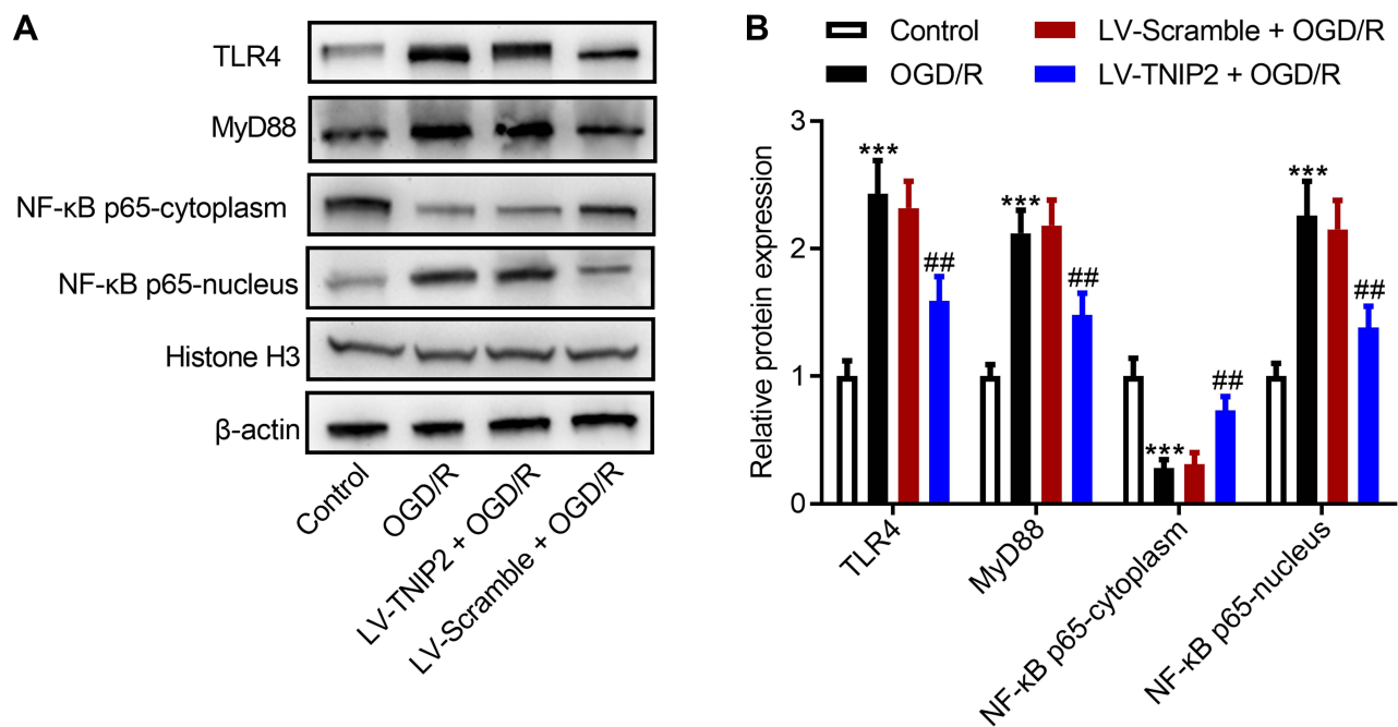
Figure 4 The TLR4/MyD88/NF- \kappa B pathway is involved in the protective effects of TNIP2 on OGD/R-induced neuronal damage. HT22 cells were transfected with LV-TNIP2 or LV-Scramble, followed by exposure to OGD/R. (A) Representative and (B) quantitative Western blot analysis of TLR4, MyD88, NF- \kappa B-cytoplasm, and NF- \kappa B-nucleus expression in HT22 cells transfected with LV-TNIP2 or LV-Scramble following OGD/R ( n = 3 ). *** P < 0.001 , compared with the control group. ## P < 0.01 , compared with the LV-Scramble + OGD/R group.
