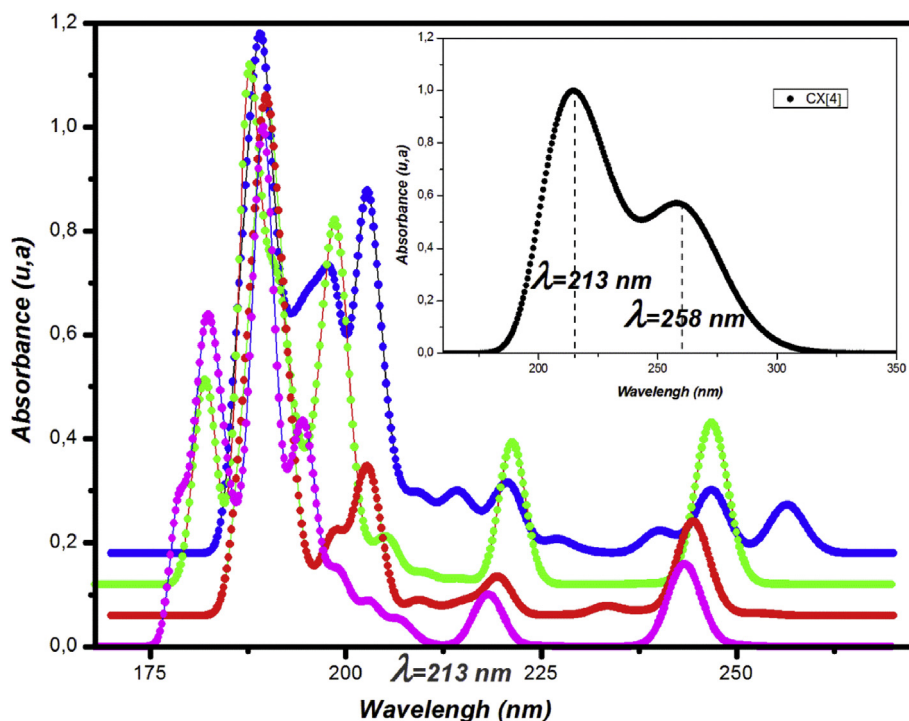
Fig. 2. Absorption spectrum of capture of TFSI - ion by calix[4]arene molecule (Blue: CX[4]-TFSI 4 , Green: CX[4]-TFSI 2 , Red: CX[4]-TFSI 1 , Magenta: CX[4]-TFSI 3 ) (according to the order of stability).
