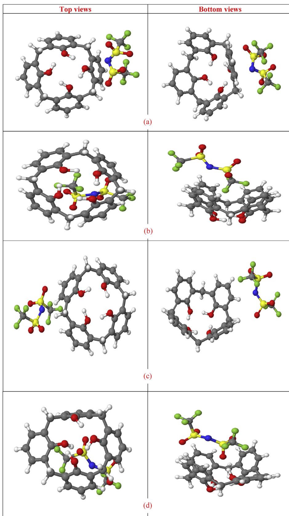
Fig. 1. Optimized geometries of and CX[4]-TFSI - (CX[4]-TFSI - 1 (a), CX[4]-TFSI - 2 (b), CX[4]-TFSI - 3 (c), CX[4]-TFSI - 4 (d)) (Top views and Bottom views) structures using B3LYP-D3/6-31+G(d) method.
