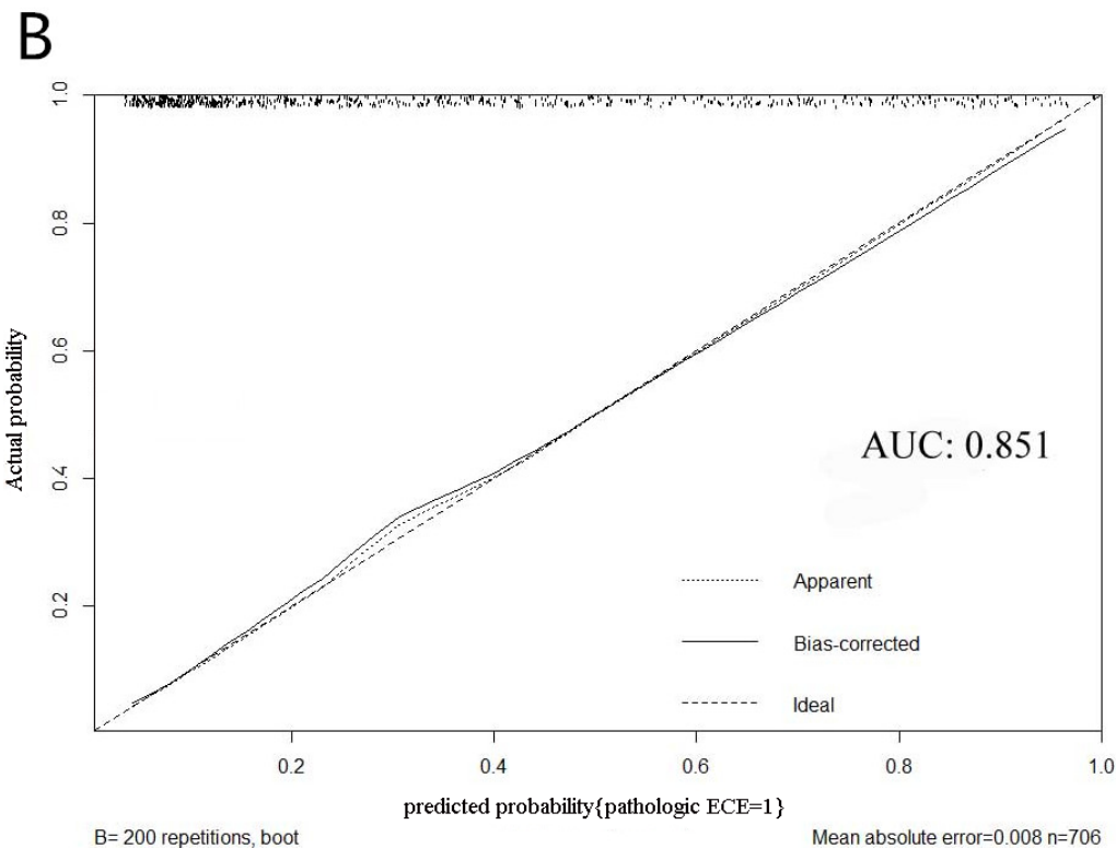
Figure 1: A. The updated nomogram predicting SS probability of ECE; B. Calibration of the nomogram (200 bootstrap re-samples).
