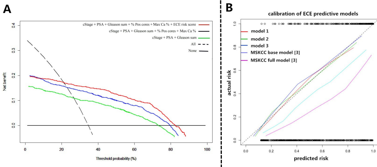
Figure 2: A. Decision curves for the three prediction models in the whole cohort. The y-axis measures net benefit, calculated by summing the benefits (true positives) and subtracting the harms (false positives), in which the latter are weighted by a factor related to the relative harm of a neglected ECE compared with the harm of missed diagnosis of ECE. A model is of clinical value if it has the highest net benefit compared with single predictors or other models. Decision analysis demonstrated a high net benefit across a wide range of threshold probabilities for the third model (red line); B. The three models of the current study were compared by MSKCC base and full models [3] for prediction of ECE by decimal of predicted risk. Better calibration was observed for the new developed models compared with MSKCC base and full models.
