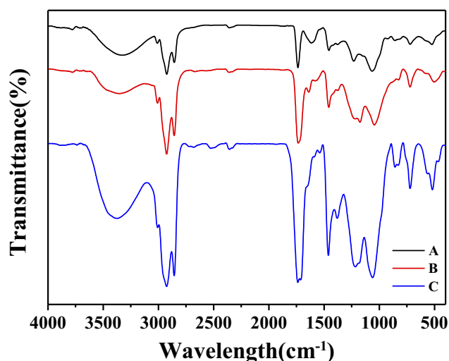
Figure 4 FTIR spectra of PE (A), PE-MAH (B) and CMC-PE (C). Abbreviations: CMC, carboxymethyl chitosan; MAH, maleic anhydride; PE, phosphatidyl ethanolamine.
