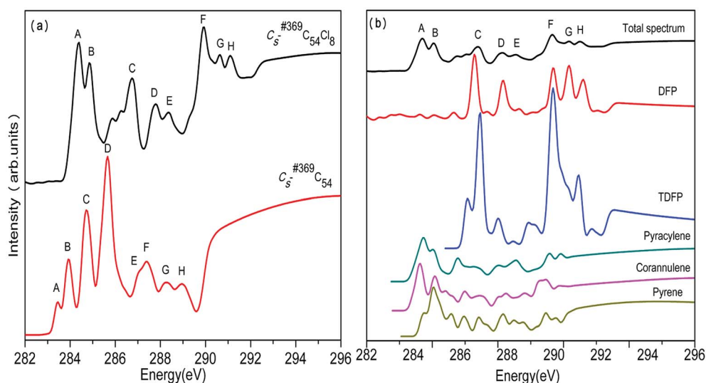
Fig. 5 Calculated (a) total NEXAFS spectra of C_s\text{-}\#369C_{54} and its corresponding chlorinated species as well as type-specific contributions for (b) C_s\text{-}\#369C_{54}Cl_8 . Each total spectrum is obtained by the weighted (according to their relative abundance) summation of all type-specific spectra.
