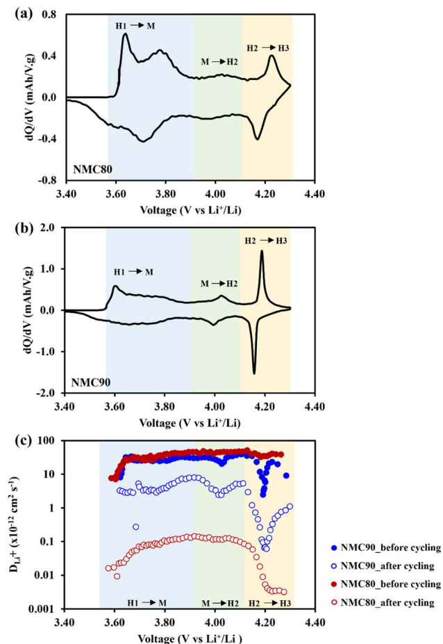
Fig. 5 dQ/dV plots at 0.1C within the voltage range 3.0–4.3 V in half-cell coin cell of (a) NMC80 and (b) NMC90 and (c) the lithium diffusivity from the GITT measurement of the NMC90 and NMC80 cells before and after 1000 cycles at 0.1C.
