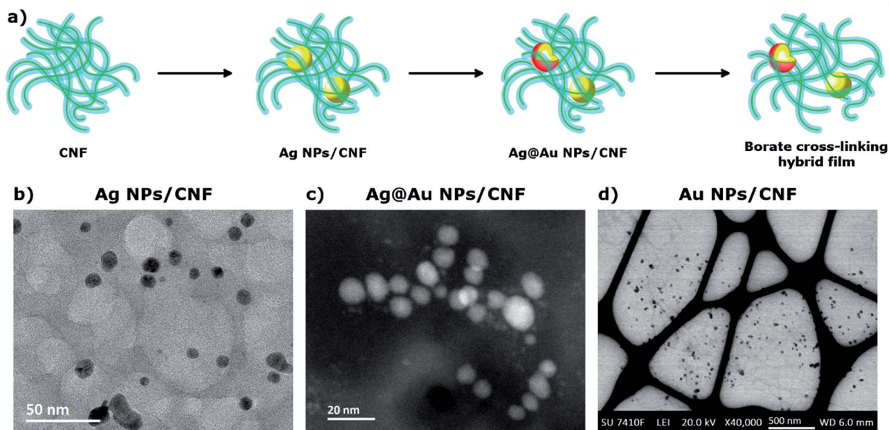
Fig. 1 (a) Representation of the synthesis of metallic and bimetallic nanoparticles with CNFs, (b) TEM image of AgNPs/CNF, (c) STEM high-angle annular dark-field image of Ag@Au NPs/CNF, and (d) STEM-in-SEM image of AuNPs supported on CNFs.
