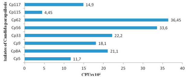
Figure 2 - Distribution of the number of cells per CFUs x 10 2 in the formation of biofilm isolates of C. parapsilosis
