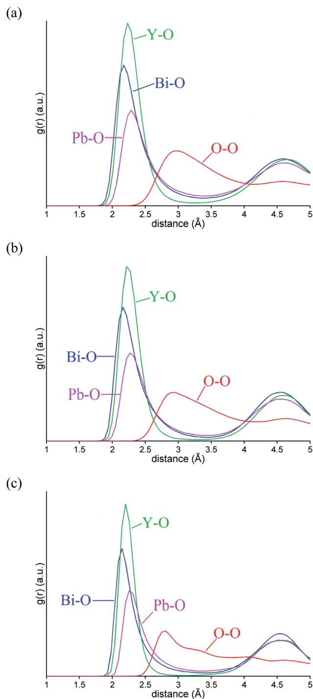
Fig. 11 Selected ion pair correlation functions g_{MO}(r) from MD simulations for \delta\text{-Bi}_5\text{PbY}_2\text{O}_{11.5} at (a) 700 °C, (b) 500 °C and (c) 25 °C showing g_{\text{BiO}}(r) (blue), g_{\text{PbO}}(r) (magenta), g_{\text{YO}}(r) (green), and g_{\text{OO}}(r) (red) distributions.
