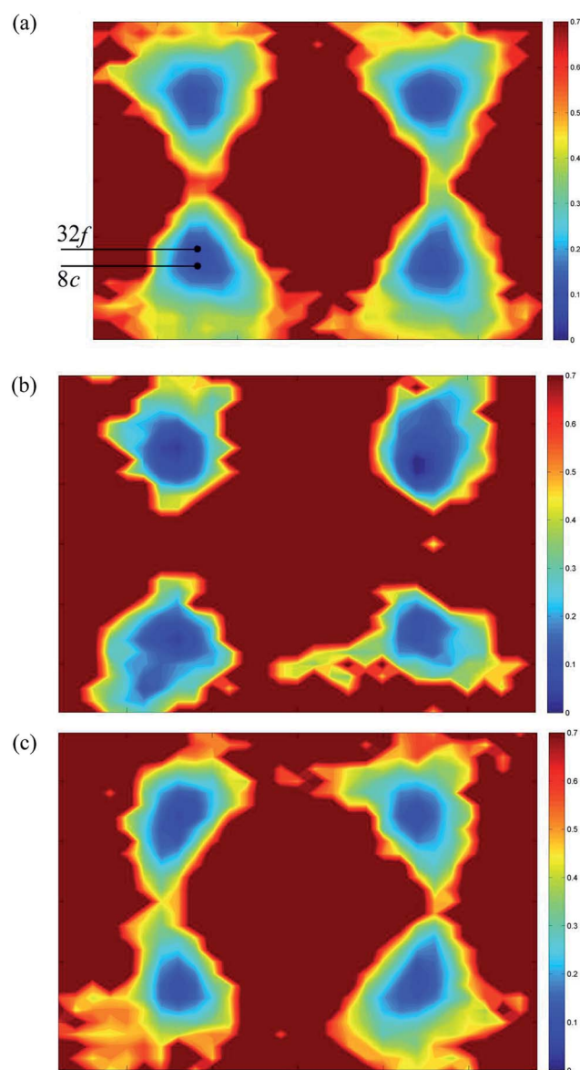
Fig. 12 (110) cross-sections of oxide-ion density around (a) \text{Bi}^{3+} , (b) \text{Pb}^{2+} and (c) \text{Y}^{3+} cations in \delta\text{-Bi}_5\text{PbY}_2\text{O}_{11.5} .
