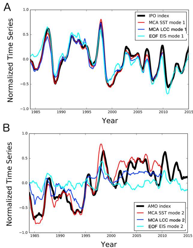
Figure 3. (a) Interdecadal Pacific Oscillation index (black) between 1984 and 2015 plotted alongside time series of the first maximum covariance analysis (MCA) mode indices for low-cloud cover (blue), sea surface temperature (red), and the first empirical orthogonal function (EOF) of estimated inversion strength (inverted, cyan). A 12-month moving average is applied to all indices. (b) Similar to (a), but for Atlantic Multidecadal Oscillation index and the second MCA/EOF modes.
