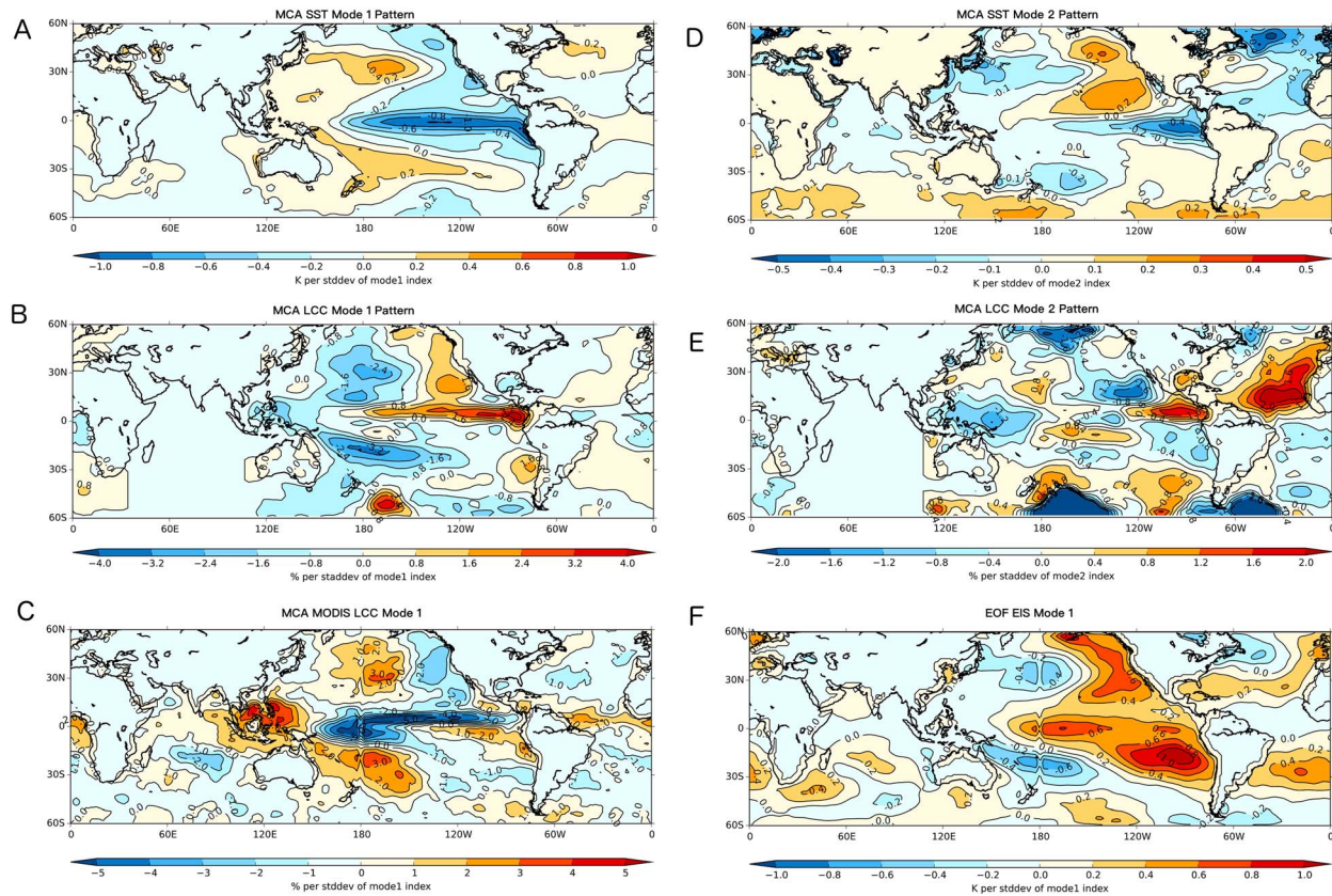
Figure 2. (a and d) Sea surface temperature anomalies corresponding to one standard deviation of expansion coefficients from maximum covariance analysis, representing Interdecadal Pacific Oscillation (IPO) and Atlantic Multidecadal Oscillation for the period 1984–2009. (b and e) The same for low-cloud cover (LCC) using International Satellite Cloud Climatology Project (ISCCP) data. (c) The same for IPO mode of LCC using MODIS data. (f) The same for estimated inversion strength using ERA-Interim during 1984 and 2009 for the IPO mode. In (a), (b), (d), and (e), the area with longitudes between 30°E and 110°E is masked out because the lack of geostationary satellite data makes the ISCCP LCC variance meaningless.
