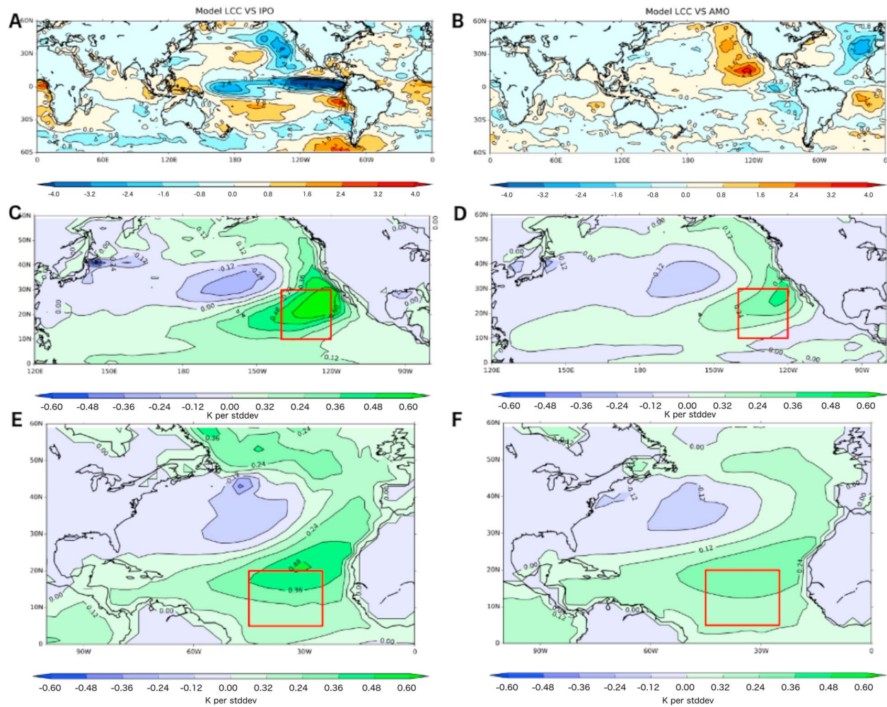
Figure 4. (a and b) Regression patterns of low-cloud cover (LCC) onto Interdecadal Pacific Oscillation and Atlantic Multidecadal Oscillation, respectively, for the HadGEM2-ES Atmospheric Model Intercomparison Project (AMIP) simulation. We compare the amplitude of internal variability of sea surface temperature (SST) in coupled historical simulations as defined in the text for models that have the (c and e) highest and (d and f) lowest SST-LCC feedback strength in AMIP simulations.
