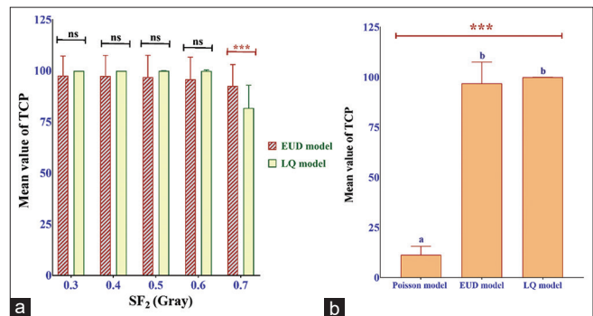
Figure 3: The mean value of computed TCP ( \pm standard deviation). (a) Comparison of TCPs between EUD and LQ models, individually for different values of SF_2 (0.3, 0.4, 0.5, 0.6, and 0.7 Gray), using paired samples t -test. (b) Comparison of TCPs in the middle group (Poisson model: \alpha/\beta = 8 , and EUD and LQ models: SF_2 = 0.5 ) among the three models. Using one-way repeated measures ANOVA with a Greenhouse–Geisser correction, followed by Bonferroni test; The groups with a similar English letter are not statistically significantly different from each other. NS = Not significant, ***P < 0.001 , and n = 30 . EUD = Equivalent uniform dose; TCP = Tumor control probability; LQ = Linear quadratic
