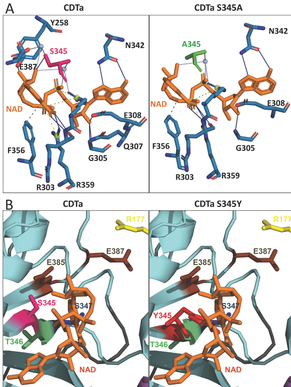
Fig 4. (A) Interaction of rCDTa and CDTa S345A with NAD. Hydrogen bonding, salt bridges, water bridges, and hydrophobic interactions are shown in blue, grey (dotted), and grey (dotted) lines respectively. Ser-345 is shown in pink and Ala-345 in green. CDTa S345A was generated using Swiss Model [20–23]. Protein ligand profiles were generated using PLIP [24]. (B) Comparison of the active sites of rCDTa and CDTa S345Y. The protein structure for rCDTa has been reported previously [13], PDB accession 2WN7. rCDTa C-terminal region is shown in cyan. NAD cofactor is shown in orange. Residue Arg-177 (ribosylation site) from the modelled Actin is shown in yellow as reference. The active site of S345Y was modelled using Swiss-Model [20–23].
