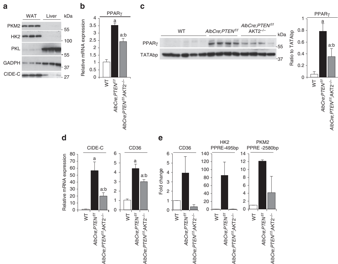
Figure 3 | PPAR \gamma controls HK2 and PKM2 expression in PTEN-null liver. (a) Immunoblot analysis of protein expression in liver and WAT tissue of WT mice. (b) RT-QPCR analysis of relative transcript levels of PPAR \gamma in the mouse livers of indicated genotypes. Data are mean \pm s.e.m., n = 5 ( P < 0.05 (a) versus WT; (b) versus AlbCre;PTEN fl/fl , 2-tailed, unpaired Student's t test). (c) Immunoblot analysis showing levels of PPAR \gamma in liver nuclear extracts. The ratio to TATA-binding nuclear protein of the densitometric assay \pm s.e.m. is presented, n = 4-5 ( P < 0.05 (a) versus WT; (b) versus AlbCre;PTEN fl/fl , 2-tailed, unpaired Student's t test). (d) Relative transcript levels of CD36 and CIDE-C in the mouse livers of indicated genotypes. Data are mean \pm s.e.m., n = 7 ( P < 0.05 (a) versus WT; (b) versus AlbCre;PTEN fl/fl ; 2-tailed, unpaired Student's t test). (e) Endogenous PPAR \gamma chromatin immunoprecipitation assessed for CD36, PKM2 and HK2 murine promoters relative to immunoprecipitation with nonspecific IgG. Data are presented as an average of fold induction over WT control mice of two independent experiments, n = 4 .
