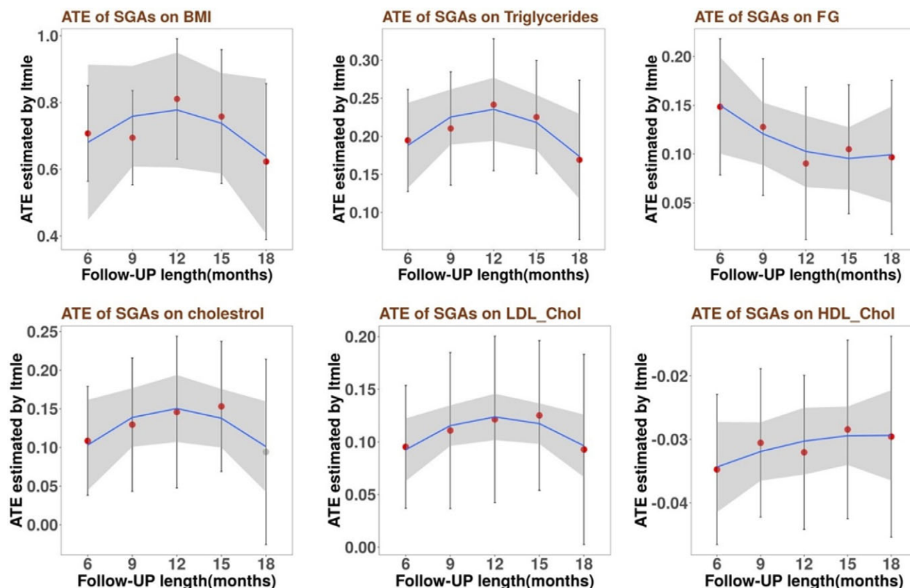
Figure 2. Average treatment effects (ATEs) of six outcomes for different FU lengths based on a 3-month interval.
