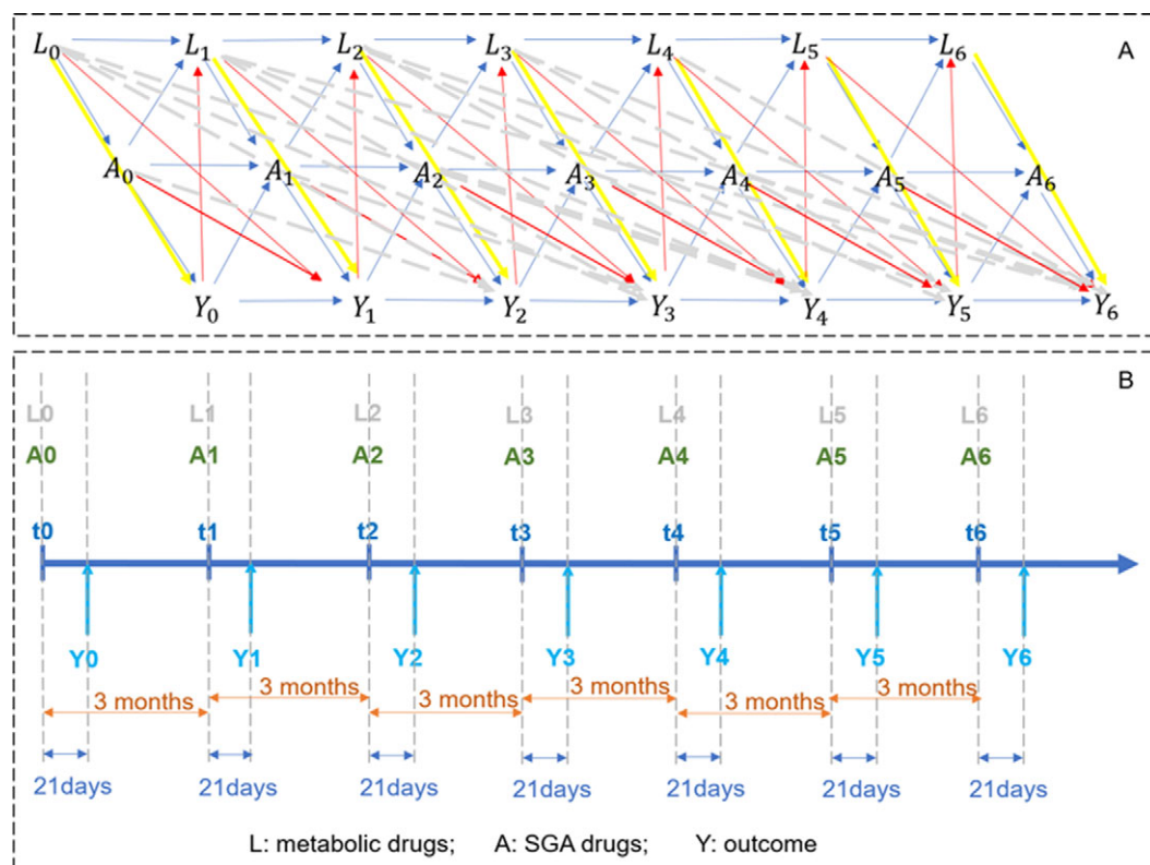
Figure 1. Assumed directed acyclic graph (A) and the sequential relationships among exposure (B), with the outcome and time-varying confounders at different time-points. L: Time-varying confounders; A: Treatment at each time-point; Y: Outcome at each time-point.
