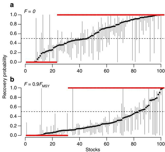
Figure 4 | Consequences of non-stationary productivity for recovery of currently depleted stocks. Shown are recovery probabilities over a 10-year timeline under no fishing ( F=0 ; a ) and under fishing at 90% of maximum sustainable yield ( F=0.9F_{MSY} ; b ). Black circles indicate probability point estimates; vertical lines display uncertainty, where the lower (upper) limit is assessed as the proportion of trajectories exceeding the 10% (90%) posterior B_{MSY} quantile. For comparison, red circles give the predicted recovery probability for each stock based on the deterministic Graham-Schaefer theory where the intrinsic productivity is fixed at its mean historical value. In the deterministic case, a stock recovers with probability 1 or 0.
