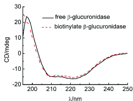
Fig. 6 CD graphs for isolated and biotinylated \beta -glucuronidase.
