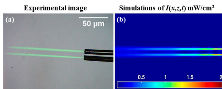
Figure 5. (a) Experimental observations (from right to left) for the SWW formed by exposure, t_{exp} = 1600 \text{ s} of \lambda = 532 \text{ nm} and P_0 = 0.1 \text{ mW} (i.e., each fiber has P_0 = 0.1 \text{ mW} ); two parallel single mode fiber optical cables; (b) simulated light intensity distributions, I(x,z,t) \text{ mW/cm}^2 .
