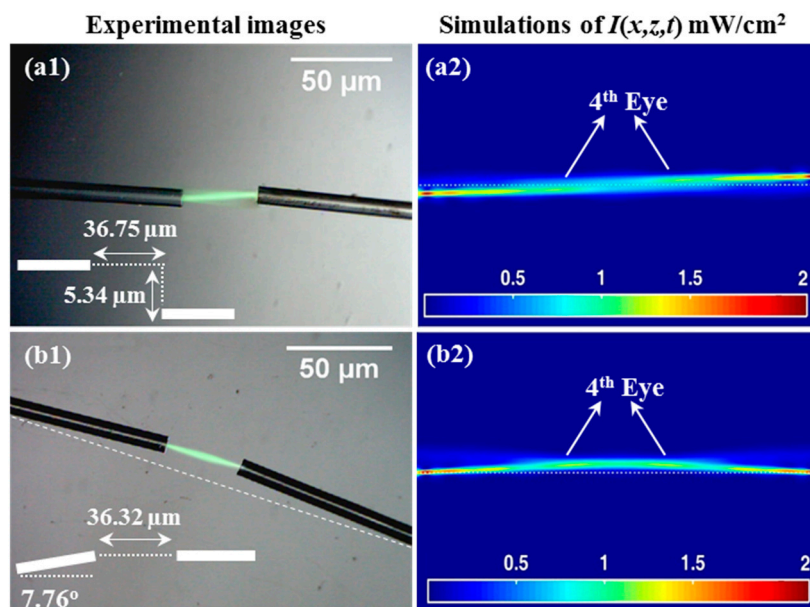
Figure 7. SWW for coupling single mode optical fibers at t_{exp} = 1600 \text{ s} of \lambda = 532 \text{ nm} and P_0 = 0.1 \text{ mW} (i.e., each fiber has P_0 = 0.1 \text{ mW} ). Experiments and simulations: (a1,a2) separated by 36.75 \mu\text{m} with shafting of 5.34 \mu\text{m} and (b1,b2) separated by 36.32 \mu\text{m} with an angle of 7.76^\circ .
