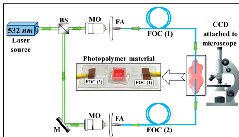
Figure 1. Optical setup for observing self-written waveguide formation through a photopolymer material to observe the dual single-mode fiber optic beam exposure.
