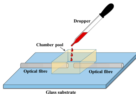
Figure 2. Drop cast photopolymer solution onto the gap between the optical fiber ends.
