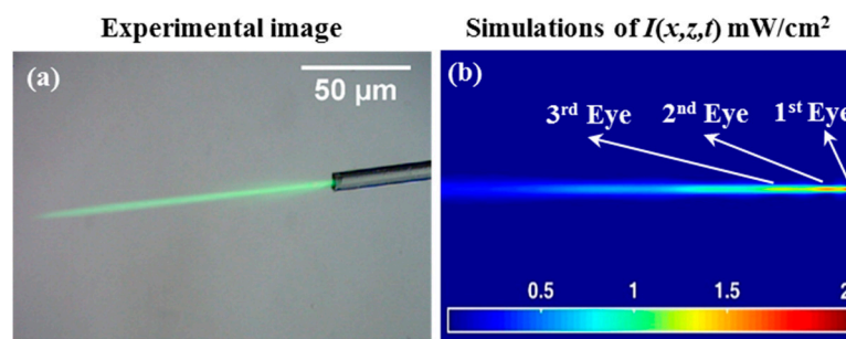
Figure 4. Light incident (from right to left) from a single mode optical fiber, t_{exp} = 1600 s of \lambda = 532 nm and P_0 = 0.1 mW: (a) experimental image results and (b) the corresponding numerical intensity predictions, I(x,z,t) mW/cm 2 .
