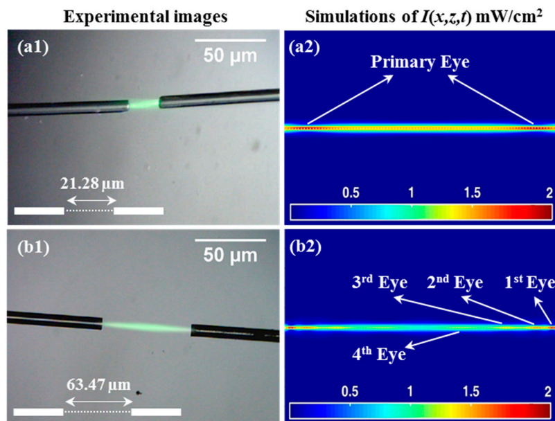
Figure 6. SWW for coupling using counter-propagation beams from single mode optical fibers. t_{exp} = 1600 s of \lambda = 532 nm and P_0 = 0.1 mW (i.e., each fiber has P_0 = 0.1 mW). The FOCs are aligned and separated by (a1,a2) 21.28 \mu\text{m} and (b1,b2) 63.47 \mu\text{m} .
