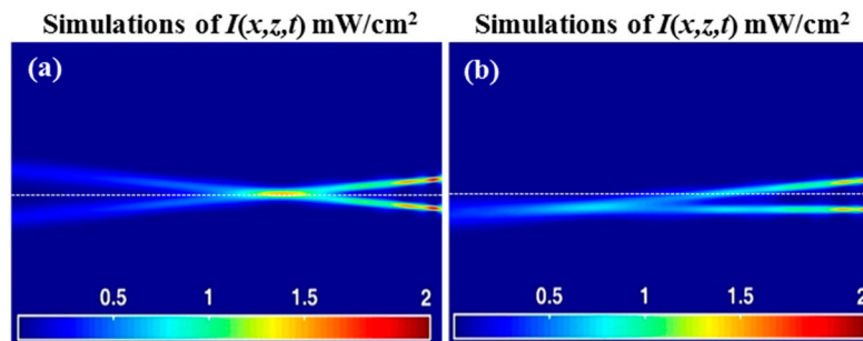
Figure 9. Predicted SWW structures, I(x,z,t) mW/cm 2 , formed at t_{exp} = 1600 s of \lambda = 532 nm and P_0 = 0.1 mW (i.e., each fiber has P_0 = 0.1 mW) for (a) the X-waveguide ( > 9^\circ ) and (b) the off-axis Y-waveguide ( < 9^\circ ).
