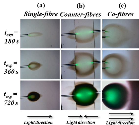
Figure 3. Microscope images of the spherical shapes created at the end of an optical fiber ( \lambda = 532 nm and P_0 = 0.1 mW) inside the liquid photosensitive solution. The three exposure geometries involve illumination using (a) single-fiber, (b) counter-fibres, and (c) co-fibres. In each case, the results for three exposure times (180 s, 360 s, and 720 s) are presented.
