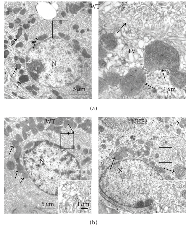
FIGURE 1: WT parietal cells (left and right). Right panel shows tubulovesicles similar to those boxed in (a). (b) Parietal cells from omeprazole treated mice: WT (left) and NHE2-/- (right). Insets show tubulovesicles from areas similar to those boxed in WT and NHE2-/- omeprazole-treated mice, respectively. Microvilli were significantly longer and the Vd of mitochondria was reduced in NHE2-/- parietal cells compared to WT. Tubulovesicles in NHE2-/- parietal cells were mostly vesicular, and often contained electron-dense cores. N: nucleus; arrowheads: mitochondria; arrows: canaliculi, boxes surround TV.
