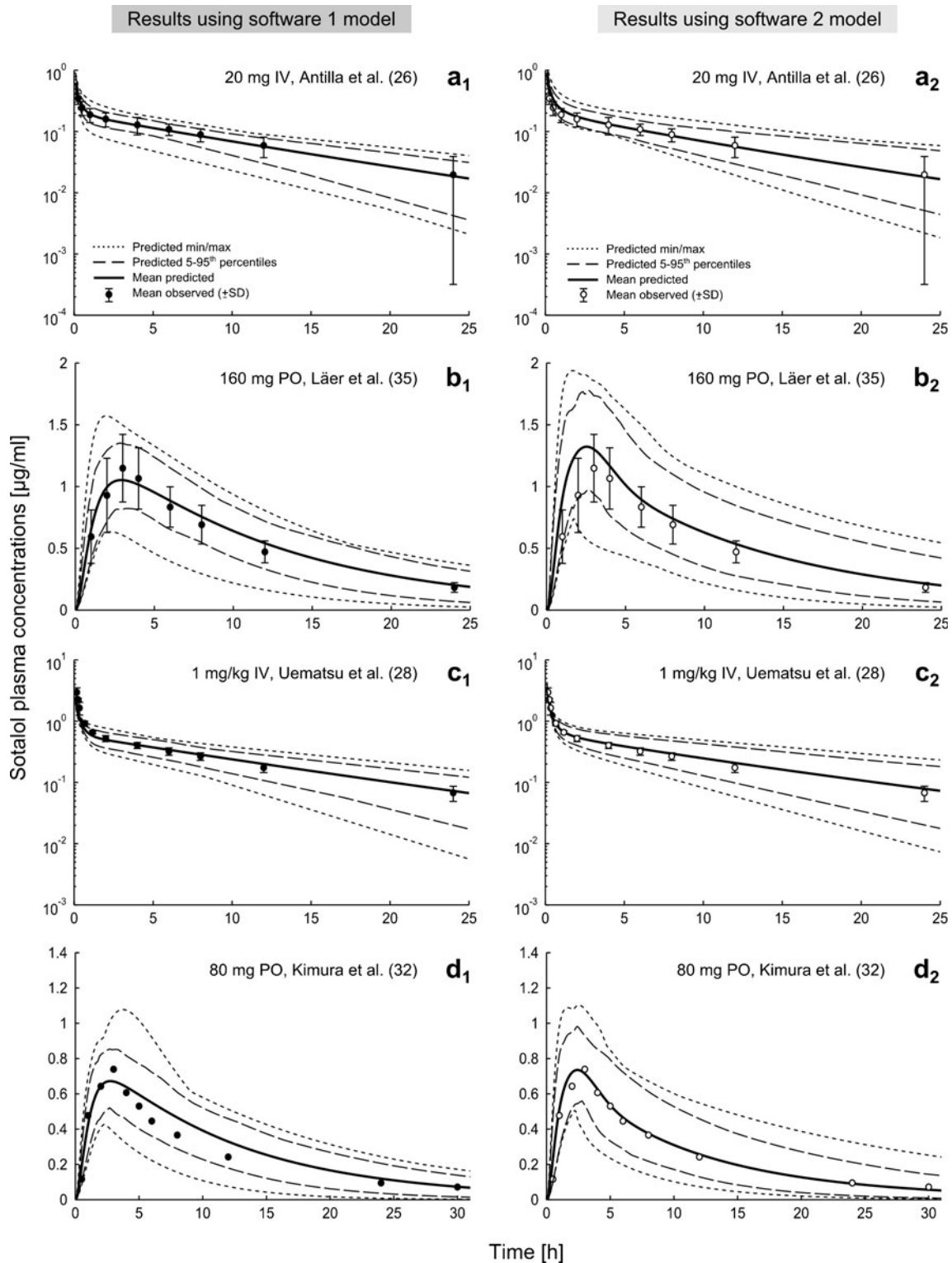
Fig. 3. Comparison of predicted ( lines ; mean, 5–95th percentiles, min/max) and mean observed ( dots ; ±SD) concentrations of IV and oral sotalolol after various dosing in both Caucasians ( a, b ) and Asians ( c, d ). Simulations were performed using software 1 (SIMCYP®, left column , filled circles ) and 2 (PK-SIM®, right column , empty circles ). Observed data are obtained from Refs. (26,28,32,35)
