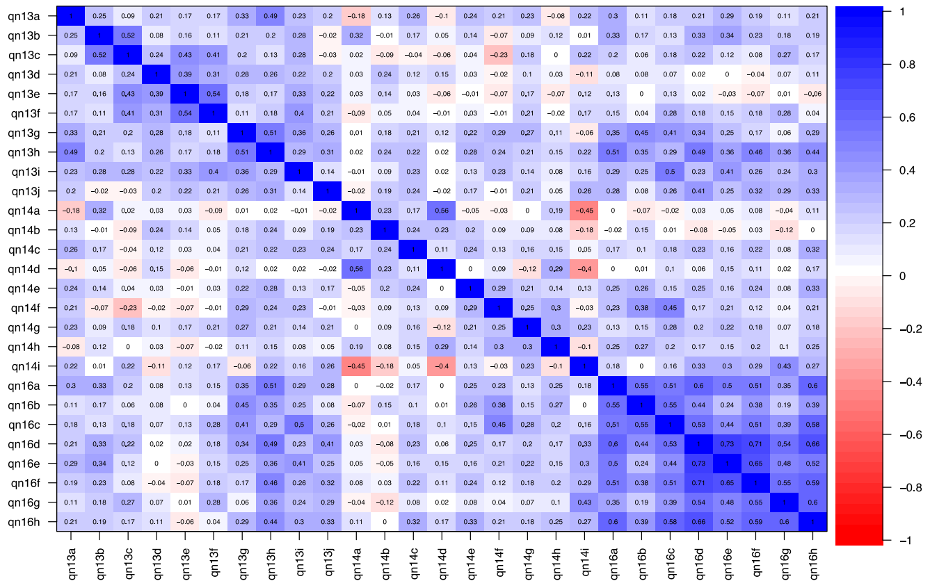
Figure 1 Correlation structure of 27 items for factors of skill practice feedback, cognitive overload, teach new skills, and assist learner’s skill acquisition.
