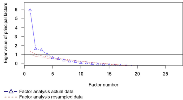
Figure 2 Parallel analysis and scree plots (Figure 1) confirmed a four-factor model existed in the P3 questionnaire.
