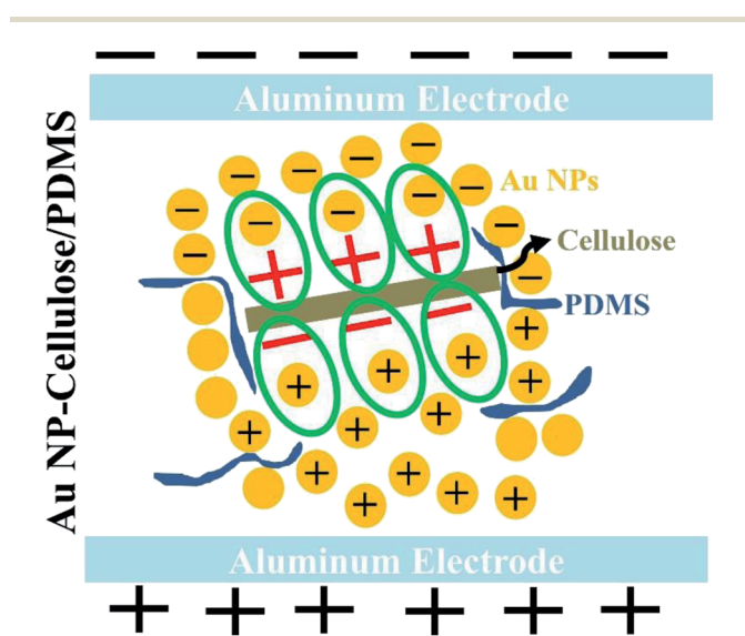
Fig. 10 Shows the schematic indicating the formation of new dipoles between Au NP–cellulose under stress and subsequently the enhancement of the piezoelectricity of the overall nanocomposite.
