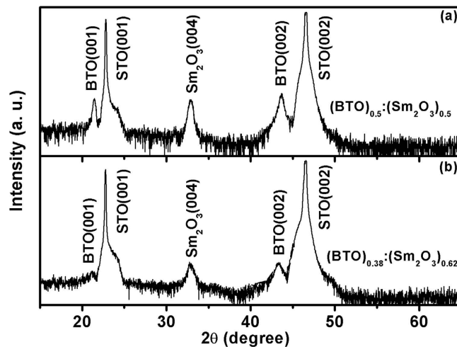
Figure 1. Comparison for the XRD \theta - 2\theta scans for BTO:Sm 2 O 3 thin films with compositions of (a) x = 0.5 and (b) x = 0.62 .
