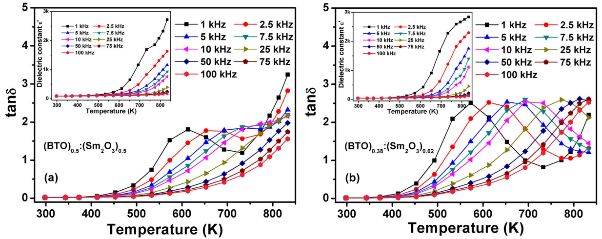
Figure 3. Temperature dependence of \tan\delta for BTO:Sm 2 O 3 thin films with (a) x=0.5 and (b) x=0.62 measured at various frequencies. The insets show temperature dependence of dielectric constant.
