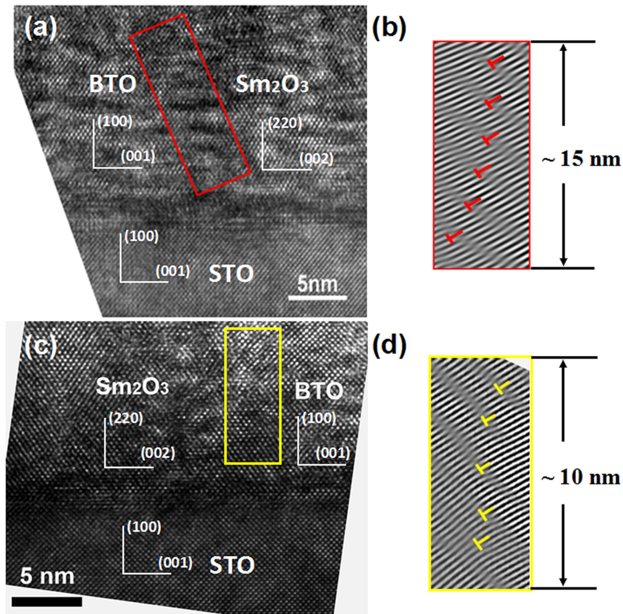
Figure 2. High-resolution TEM images of BTO:Sm 2 O 3 thin films with (a) x = 0.5 and (c) x = 0.62 . Corresponding Fourier-filtered (FFT) images along column boundaries are shown as (b) and (d), respectively. The FFT images are enlarged to show misfit dislocations clearly.
