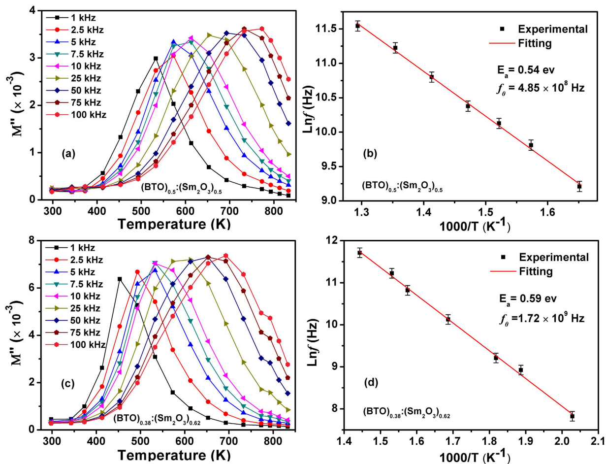
Figure 5. Variation of M'' as a function of temperature for BTO:Sm 2 O 3 thin films with (a) x=0.5 and (c) x=0.62 measured at different frequencies. The corresponding Arrhenius plots of the frequency against temperature were shown in (b) and (d), respectively. The solid curves are the best fits to the Arrhenius law.
