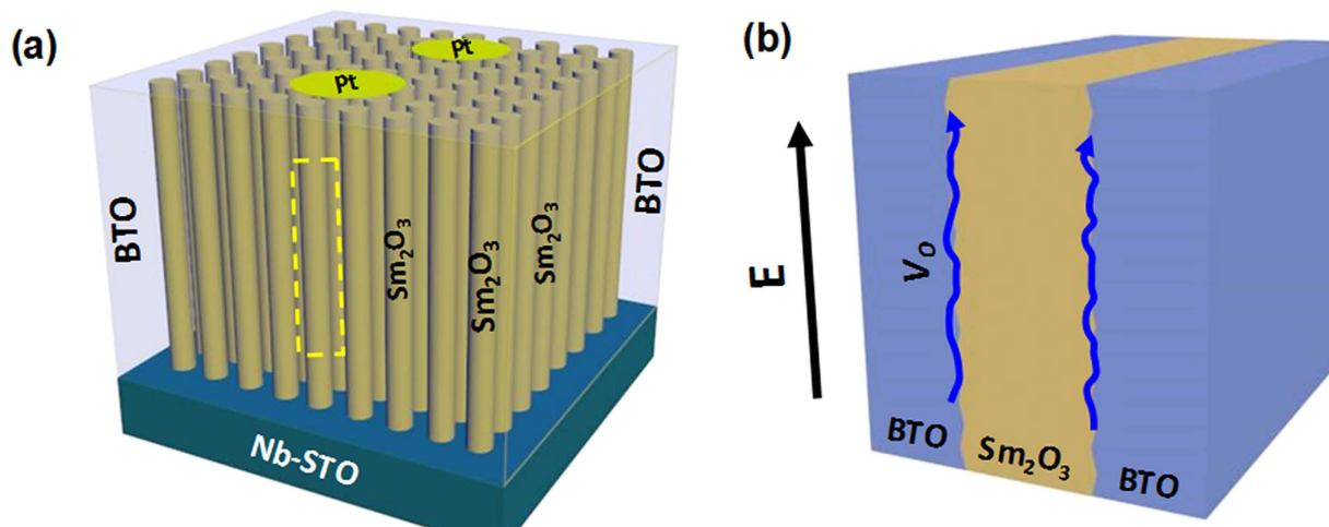
Figure 6. (a) Schematic diagram of Pt/BTO:Sm 2 O 3 /Nb-STO vertical sandwich capacitors. (b) The expanded view of the dashed part in the schematic diagram to show the interfaces between Sm 2 O 3 nanocolumns and BTO matrix. E and blue lines represent the electric field and the pathway of movement of V O s, respectively.
