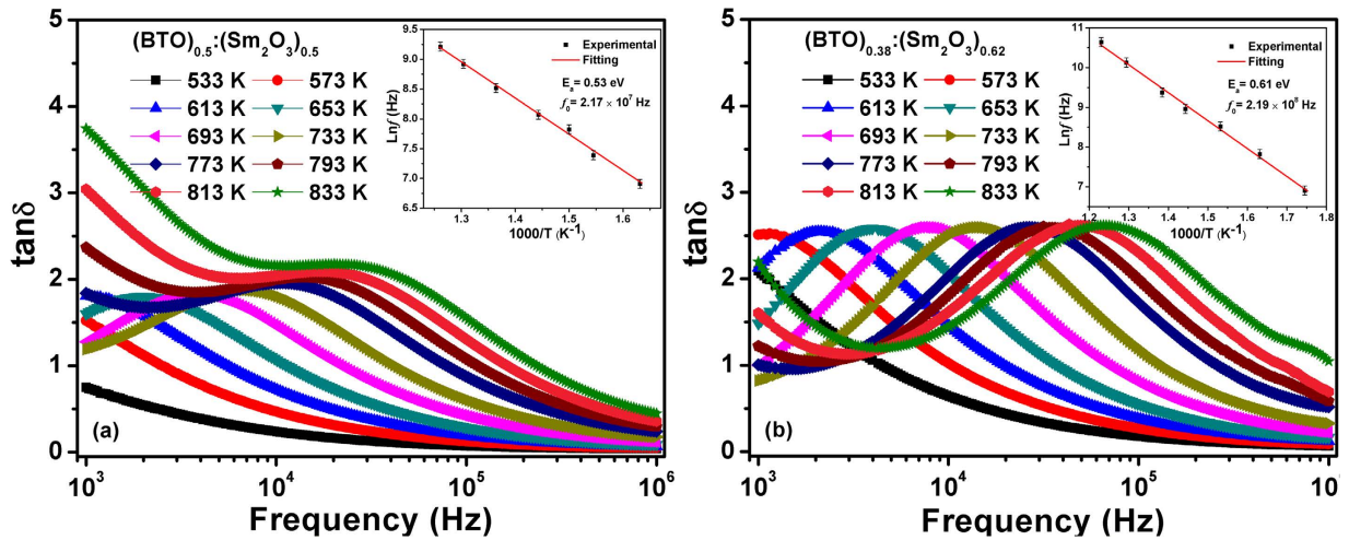
Figure 4. Frequency dependence of \tan\delta for BTO:Sm 2 O 3 thin films with (a) x=0.5 and (b) x=0.62 measured at different temperatures. The insets show the Arrhenius plots of relaxation times. The red straight lines in insets are the linear fitting based on the Arrhenius law.
