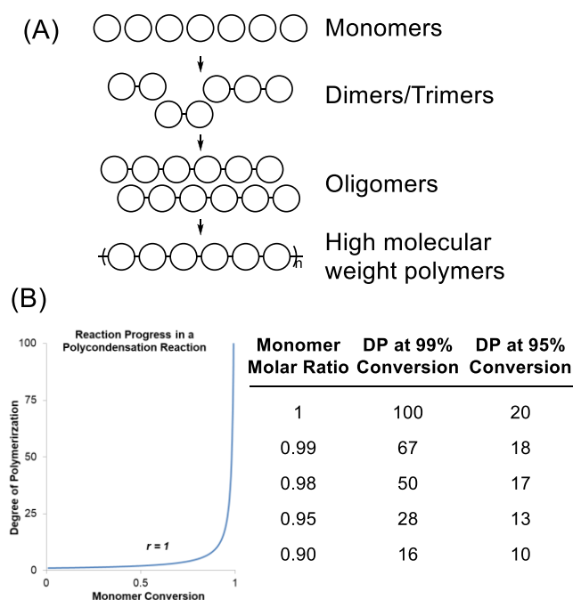
Figure 1. Qualitative and quantitative representations of polycondensation reactions.
