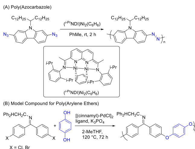
Scheme 14. Representative Polymers Prepared from Aryl Azides and by C–O Cross-Coupling a
