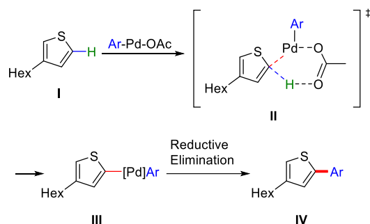
Scheme 2. CMD-Mediated Direct Arylation
