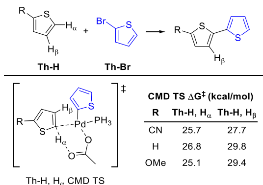
Scheme 4. Activation Free Energies for CMD of Substituted Thiophenes a
