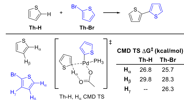
Scheme 5. Activation Free Energies for CMD of Thiophene a
