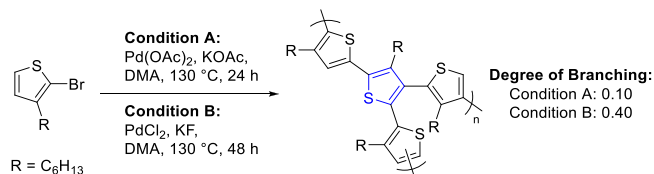
Scheme 6. Hyperbranched P3HT a
