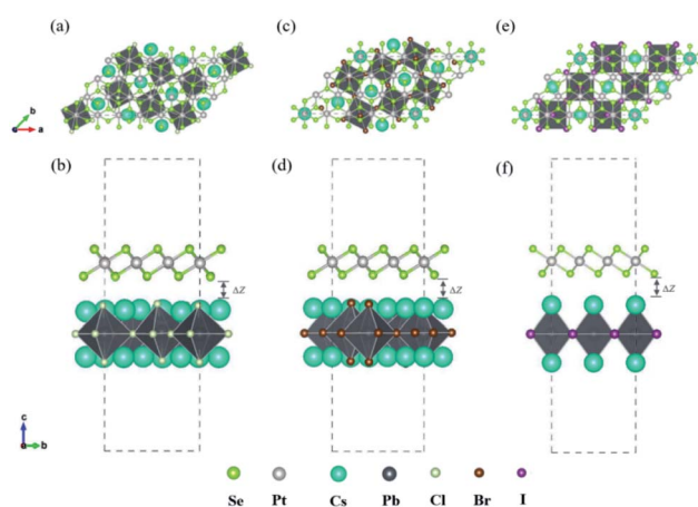
Fig. 1 Top and side views of relaxed 45° Cs 2 PbX 4 –PtSe 2 heterostructures. (a and b) Cs 2 PbCl 4 –PtSe 2 heterostructure. (c and d) Cs 2 PbBr 4 –PtSe 2 heterostructure. (e and f) Cs 2 PbI 4 –PtSe 2 heterostructure. The unit cell of Cs 2 PbX 4 –PtSe 2 heterostructures are made up of \sqrt{10} \times \sqrt{5} cubic phases Cs 2 PbCl 4 and 5 \times \sqrt{13} PtSe 2 , \sqrt{10} \times \sqrt{5} cubic phases Cs 2 PbBr 4 and 5 \times \sqrt{13} PtSe 2 , and \sqrt{8} \times 2 cubic phases Cs 2 PbI 4 and 5 \times \sqrt{13} PtSe 2 , as shown in figure.
