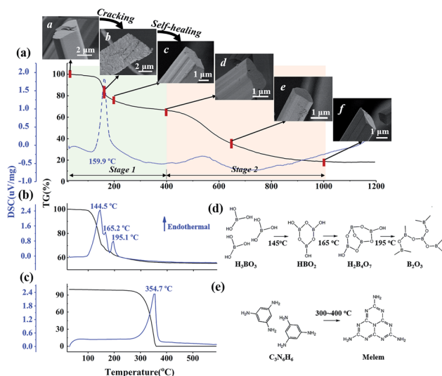
Fig. 1 TG-DSC curves of (a) M·2B supramolecular fibers, (b) H_3BO_3 and (c) C_3N_6H_6 . In (a), the first weight-loss stage is in the range of 20–400 ^\circ\text{C} ; the second weight-loss stage is in the range of 400–1000 ^\circ\text{C} , the inset SEM images demonstrate the morphological evolution of the C_3N_6H_6 \cdot 2H_3BO_3 fibers during thermal treatment: a M·2B, b M·2B 150 , c M·2B 200 , d M·2B 400 , e M·2B 650 , f M·2B 1000 . (d) Molecular transformation of H_3BO_3 and (e) C_3N_6H_6 in the heating process. In (d), H_3BO_3 is converted to metaboric acid ( HBO_2 ) and further to tetraboric acid H_2B_4O_7 and finally to a boron oxide structure. In (e), C_3N_6H_6 condenses to melem at 300–400 ^\circ\text{C} . 22
