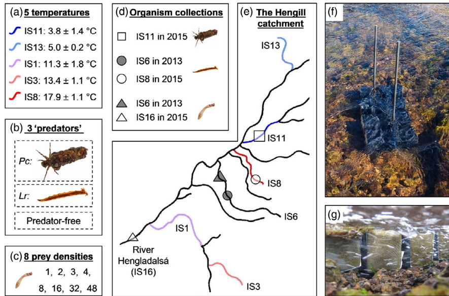
FIGURE 1 Overview of the field experimental design: (a) five stream temperatures (mean \pm SD); (b) three predator treatments, including the cased caddisfly larva Potamophylax cingulatus ( Pc ), the housefly larva Limnophora riparia ( Lr ) and a predator-free control; and (c) eight prey densities of the blackfly larvae (Simuliidae). (d) The stream each taxon was collected from in each year of the experiments. (e) Map of the Hengill geothermal stream catchment, highlighting the streams where the experimental microcosms were deployed for the field experiments, with colours and labels corresponding to (a), and where the organisms used in the experiments were collected, with symbols corresponding to (d). Note that the mean temperatures of IS6 and IS16 during organism collections were 17.4°C and 7.5°C, respectively. Microcosms in situ in (f) plane and (g) side elevation
