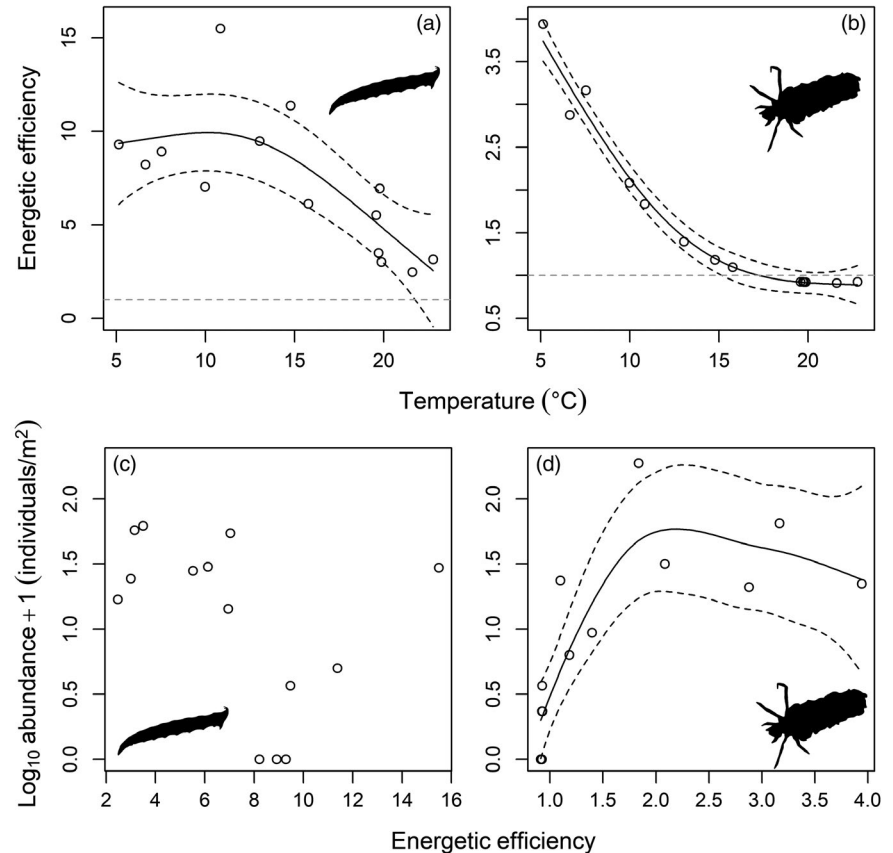
FIGURE 6 Relationships between energetic efficiency and temperature for (a) Limnophora riparia and (b) Potamophylax cingulatus feeding on natural densities of Simuliidae from 14 streams of different temperature in the Hengill catchment. Data points above and below the dashed grey line indicate scenarios where energy intake is greater than ( y > 1 ) and less than ( y < 1 ) energy expenditure, respectively. Energetic efficiency was a poor predictor of population abundance in (c) L. riparia , but it was an excellent predictor of population abundance in (d) P. cingulatus . Solid lines are the significant relationships from generalized additive models, and dashed lines are the 95% confidence intervals of model fittings
