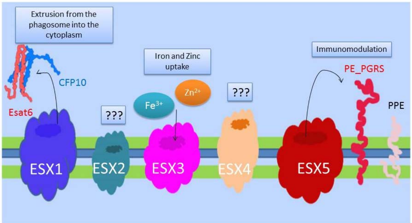
Figure 1 - Protein Secretion systems. Five different secretion system have been described in Mtb (titled Type VII Secretion System -T7SS), encoded by gene clusters and called ESX1 to ESX5. ESX1 and ESX5 secrete different proteins involved in the virulence of Mtb : ESX1 secretes antigens that interfere with the integrity of the phagosomal membrane, leading to phagosomal rupture and bacterial emission into the cytosol. ESX5 is present only in slow growing mycobacteria (such as Mtb and M. marinum ) and it is thought to be involved in the secretion of proteins (PPE and PE-PGRS) with immunomodulatory properties. ESX3 is involved in Zinc and Iron uptake and homeostasis and as such is essential for growth. The role of ESX2 and ESX4 remain still unknown.
