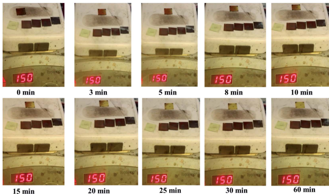
Fig. 4 Images of perovskite films annealed at 150 °C in glove box ( N_2 ). The front row shows only MAPbI 3 . The second row (from left to right) shows CsPbI 3 , CsPb 0.75 Sn 0.25 I 3 , CsPb 0.5 Sn 0.5 I 3 , CsPb 0.25 Sn 0.75 I 3 , and CsSnI 3 .
