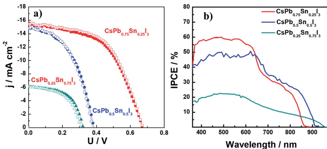
Fig. 5 (a) The J - V curves obtained under full sun illumination for devices based on CsPb 0.75 Sn 0.25 I 3 , CsPb 0.5 Sn 0.5 I 3 , and CsPb 0.25 Sn 0.75 I 3 as photoactive layers with ITO/PEDOT/PVSK/PCBM/bis-C 60 /Ag configuration. (b) Their incident photon-to-current conversion efficiency spectra. All the samples were tested without extra protection or encapsulation.
