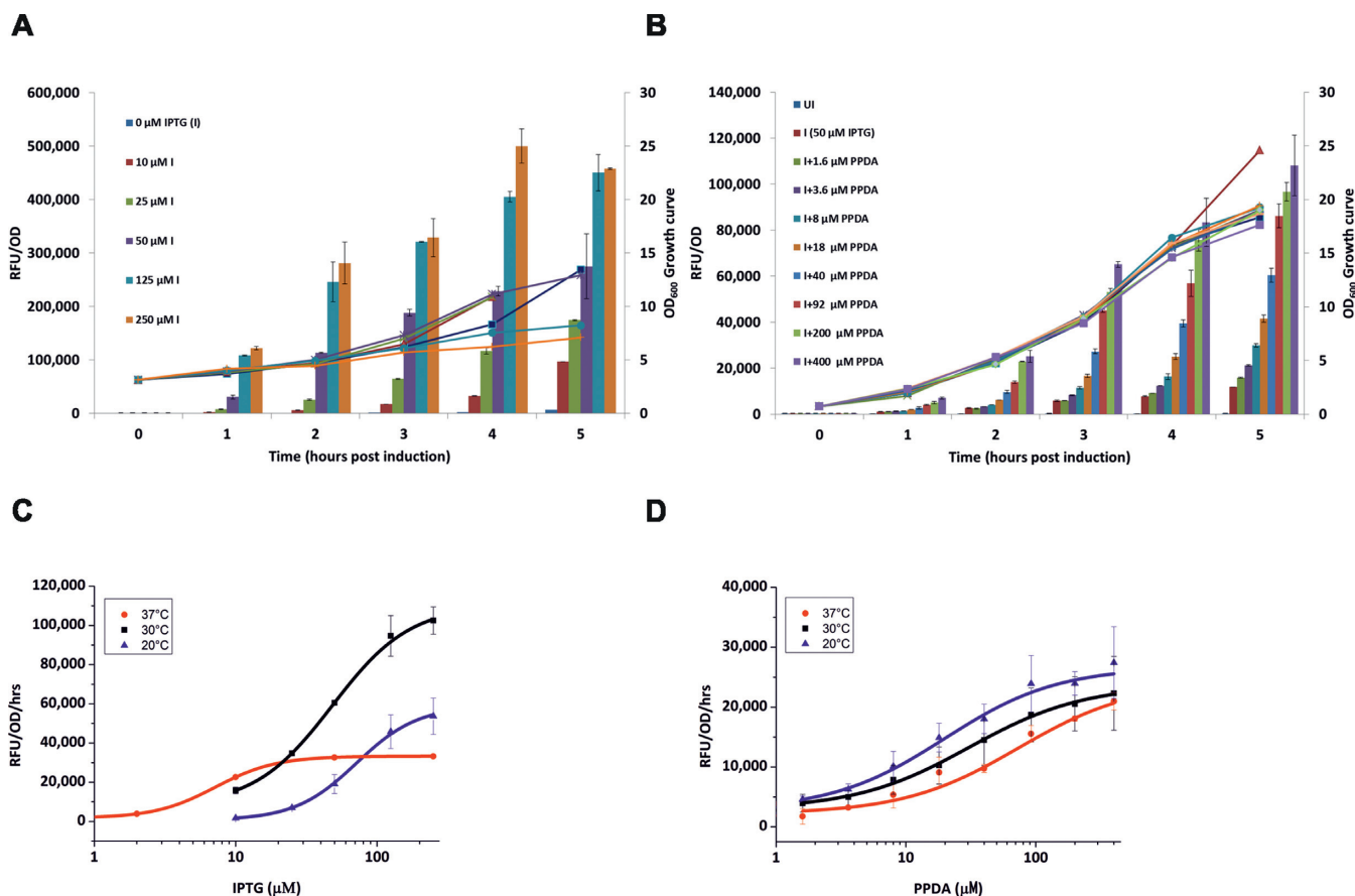
Figure 3. High cell density expression kinetics and performance. The t/t and rT/rT systems were grown at 30°C in 125 ml baffled flasks and induced when in log phase with the indicated concentrations ( \mu\text{M} ) of IPTG (I) and PPDA (P). Samples were collected at different times post induction and analysed for eGFP expression. A–B , normalized expression RFU/OD 600 (bars) and absolute OD 600 values (lines) were then plotted versus time for the t/t (A), and the rT/rT systems (B). (C–D) kinetic dose-response data fitted with a four-parameter logistic function of the RFU/OD values at different time points and induction temperatures for the t/t system titrated with IPTG (C), and the rT/rT system titrated with PPDA at a fixed IPTG concentration of 50 \mu\text{M} (D). The data represent the mean of at least two replicates with error bars showing standard errors.
