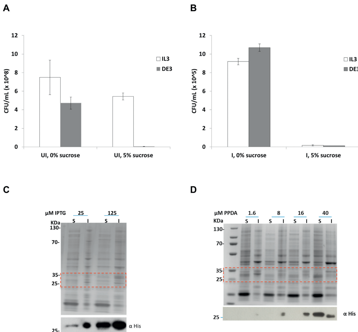
Figure 5. Expression of toxic and challenging proteins. (A–B) Comparison of colony-forming unity (CFU) from sacB assay, CFU/ml counts for both t/t and tT/tT systems carrying a pET15- sacB plasmid were determined in the absence (A) and presence (B) of inducers with and without the addition of 5% sucrose. In the absence of inducers (UI), expression of the sacB gene led to highly sucrose-sensitive behaviour in the t/t system, whereas upon induction (I/P, 50 μM IPTG plus 100 μM PPDA) both systems displayed sensitivity. The data represent the mean of at least three replicates with error bars showing standard deviation errors. (C–D) solubility analysis of the scFv protein, visualized by SDS-PAGE and western blot, of soluble (S) and insoluble (I) fractions. t/t was induced for 3 h at 30°C (C) and tT/tT for 20 h at 30°C (D), with the indicated concentration of inducer.
