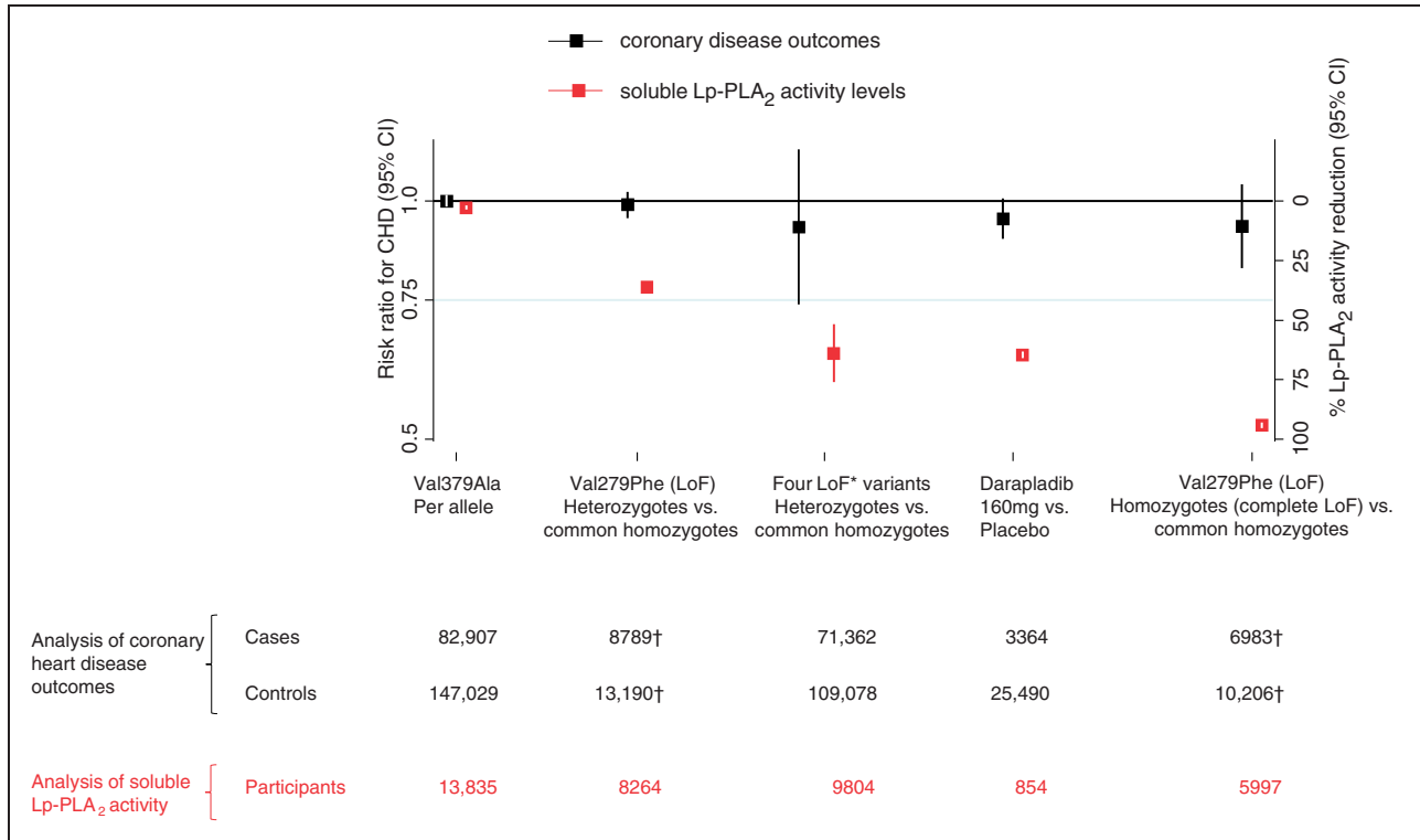
Figure 3. Association of Lp-PLA 2 -lowering alleles with Lp-PLA 2 activity and CHD risk.
