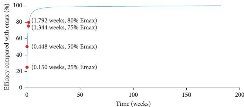
FIGURE 5: Model prediction.
