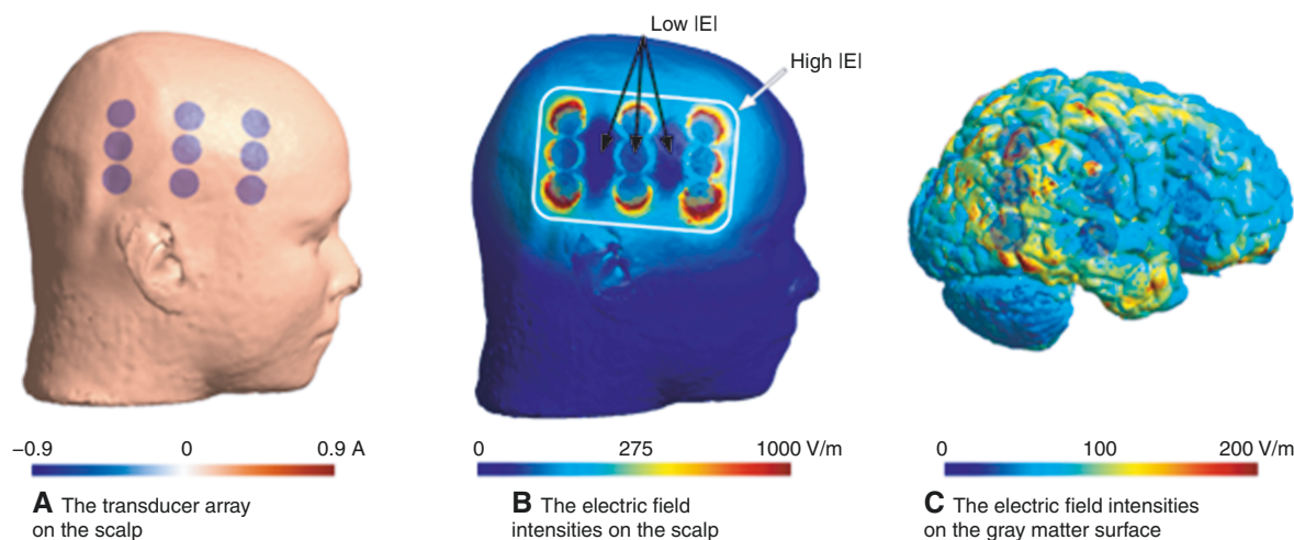
Figure 6. A single electrode array is shown in figure (A–C) shows the corresponding electric field intensity, which is highest around the edges and lowest in the center illustrating the “edge effect.” Color-coded field intensity map in V/m. For example, a tumor located directly underneath the center electrode would experience lower field intensities and the transducer array could be moved accordingly so that the edges of the transducer arrays overlap the pathology for maximum field intensity.
